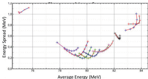
Figure 3: Energy Spread as a function of Average Energy for a variation of the phase of 4 cavities. Each line represents one case with 3 cavity phases fixed and the phase of the remaining cavity varied.
