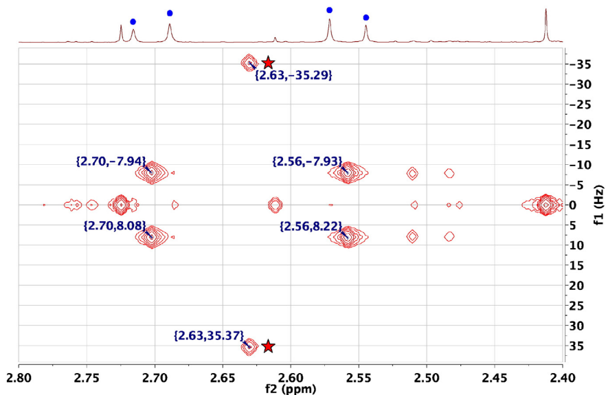
Fig. 8. An expansion of the 600 MHz 2D ^1\text{H} -resolved NMR spectrum of the urine of a male, 30-week-old, FMO5 knockout mouse [61] in the region of the AB resonances from citric acid at ca 2.70 and ca 2.56 ppm (four dots in 1D spectrum), displayed as a contour plot underneath the corresponding 1D ^1\text{H} NMR spectrum. The spectrum is tilted by 45^\circ , so that all the signals of each multiplet appear at the same chemical shift, and symmetrised. The signals labelled with stars, appearing at ca 2.63 ppm, exactly in between the shifts of the two citrate signals are 2nd order effects caused by the mixing of transitions between the A and B spins by the 180^\circ pulse, in the presence of strong coupling. As is clear from the 1D ^1\text{H} NMR spectrum, there are no real signals at 2.63 ppm!
