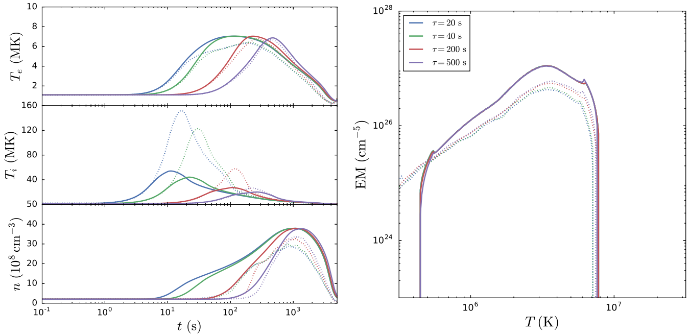
Figure 5. Two-fluid EBTEL simulations for \tau = 20, 40, 200, 500 s in which only the ions are heated. Left: Electron temperature (upper panel), ion temperature (middle panel), and density (lower panel). Right: Corresponding EM(T) calculated according to Section 3. The pulse durations and associated colors for all panels are shown on the right. All parameters are the same as those discussed in Section 3.1.1. In all panels, the solid (dotted) lines show the corresponding EBTEL (HYDRAD) results.
