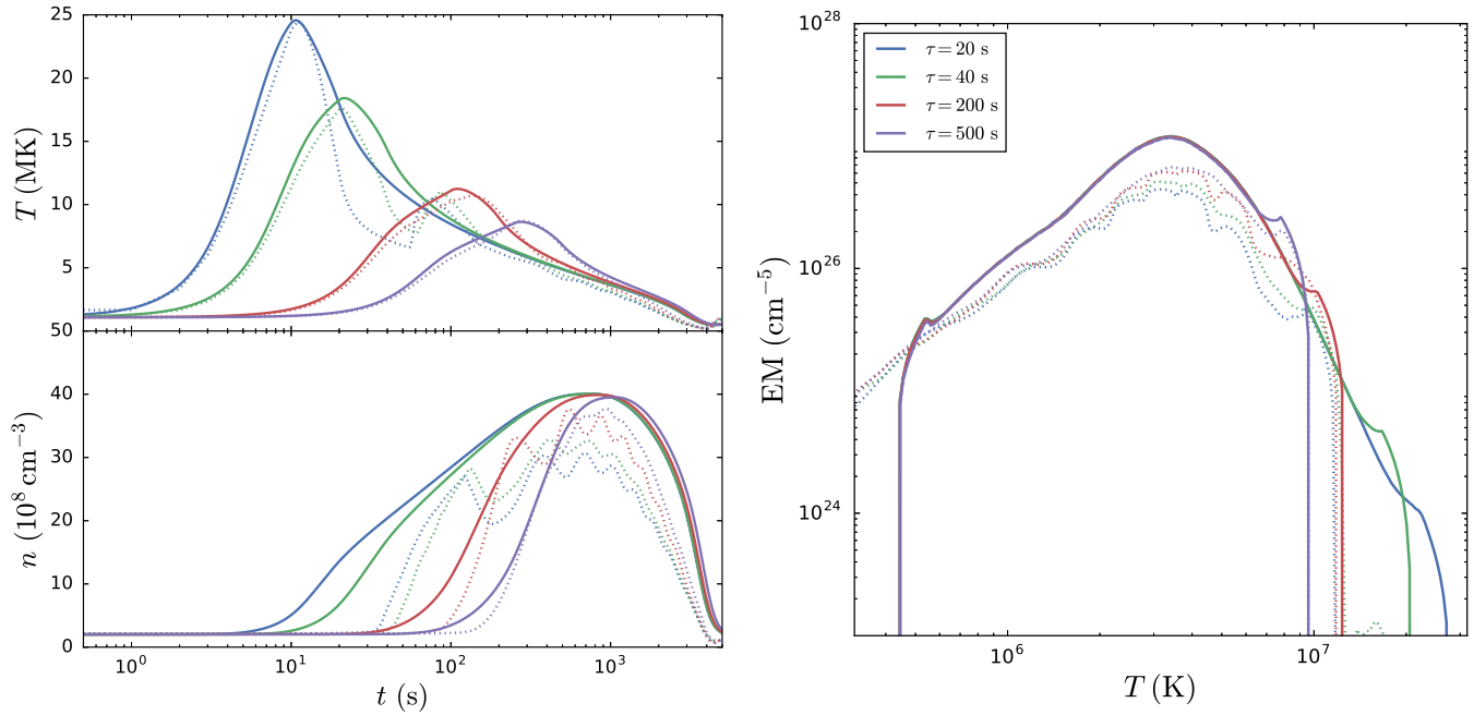
Figure 1. Left: Temperature (upper panel) and density (lower panel) profiles for a loop with 2L = 80 Mm. Each heating profile is triangular in shape with a steady background heating of H_{bq} = 3.5 \times 10^{-5} ergs \text{cm}^{-3} \text{s}^{-1} . The duration of the heating pulse is varied according to \tau = 20, 40, 200, 500 s, with each value of \tau indicated by a different color, as shown in the right panel. The total energy injected into the loop is fixed at 10 ergs \text{cm}^{-3} . Note that time is shown on a log scale to emphasize the behavior of the heating phase. Right: Corresponding \text{EM}(T) for each pulse duration \tau . The relevant parameters and associated colors are shown in the legend. \text{EM}(T) is calculated according to the procedure outlined in the beginning of Section 3. In all panels, the solid (dotted) lines show the corresponding EBTEL (HYDRAD) results (see Section 3.1.2).
