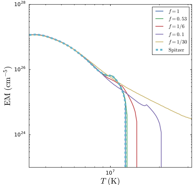
Figure 2. EM(T) calculated from the single-fluid EBTEL model when only pure Spitzer conduction is used (turquoise, dashed) and when a flux limiter is imposed according to Section 2.1. In the free-streaming limit, five different values of f are considered (see legend). The pulse duration is \tau = 200 s. All other parameters are the same as those discussed in Section 3.1.1. Note that here we only show EM(T) for T > T_m as the cool side of EM(T) is unaffected by our choice of f .
