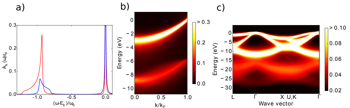
FIG. 1. a) GW plus cumulant spectral functions of the three-dimensional electron gas at \mathbf{k} = 0 for r_s = 1.0 (red curve) and r_s = 3.0 (blue curve). b) Spectral functions (in 1/\text{eV} ) of the three-dimensional electron gas at r_s = 4.0 (corresponding to metallic sodium) from GW plus cumulant theory. c) Spectral functions (in 1/\text{eV} ) of silicon from ab initio GW plus cumulant theory calculations.
