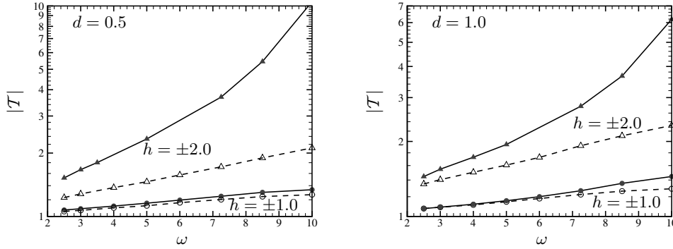
FIGURE 9. Transmission coefficients |T| vs. \omega for different h and d = 0.5 (left figure), 1.0 (right figure). Solid lines with filled symbols are for humps; dashed lines with open symbols are for indentations.
