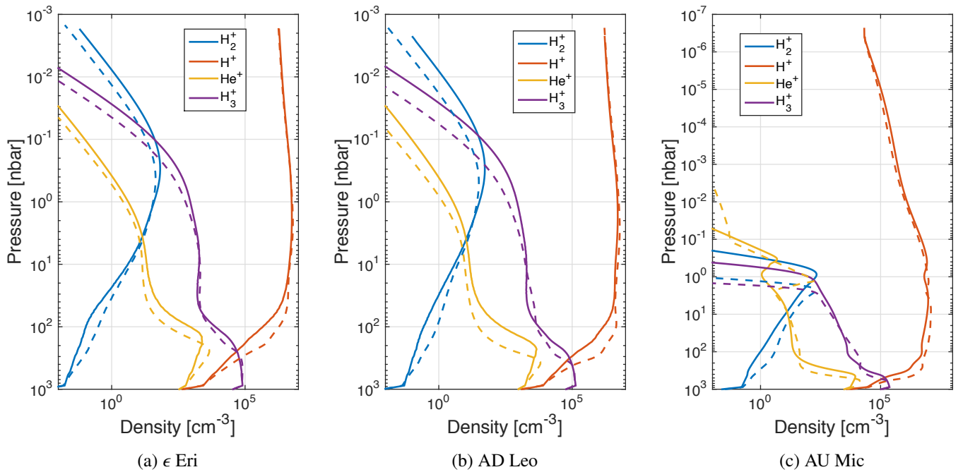
Fig. 10. Ion densities as a function of pressure at 30° latitude and 12 LT for an EGP irradiated by the synthetic spectra (solid lines) and the scaled solar spectra (dashed lines). The orbital distance is 1 AU.
