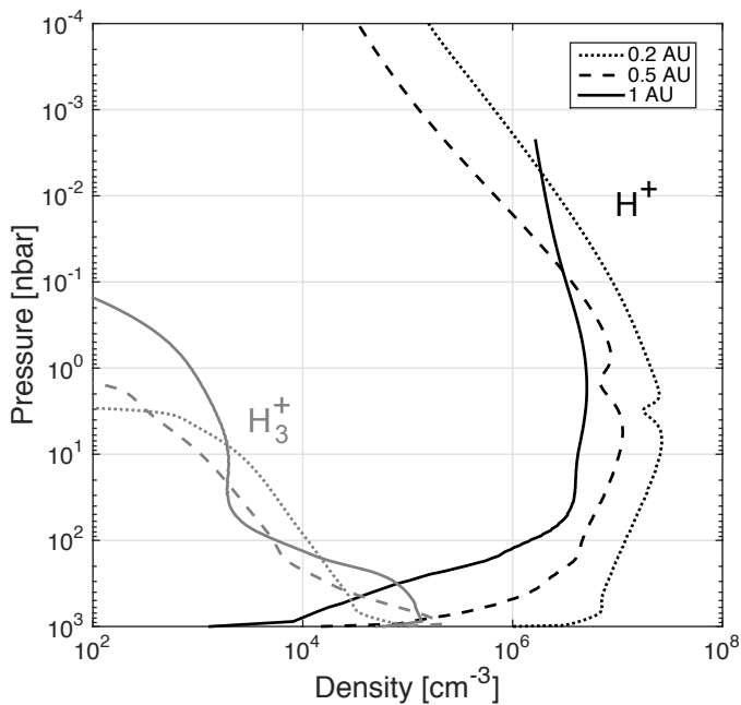
Fig. 9. Major ion densities for an EGP orbiting AD Leo at different orbital distances, determined at 30° latitude and 12 LT.
