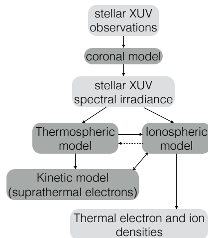
Fig. 1. Schematic of model elements (dark grey boxes) and inputs/outputs (light grey boxes).
