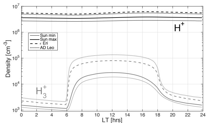
Fig. 6. Diurnal variation of peak H^+ (in black) and H_3^+ (in grey) densities in an EGP orbiting the Sun at solar minimum (thin solid lines), the Sun at solar maximum (thick solid lines), the star \epsilon Eri (dashed lines), and the star AD Leo (dotted lines).
