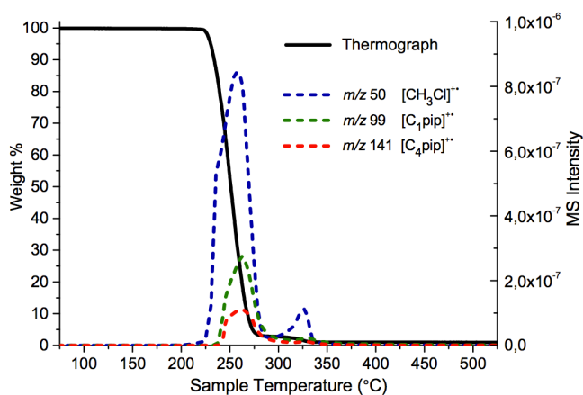
Fig. 8 TGA-MS evaluation of [C_4C_1pip]Cl , 2 . The continuous line denotes the TGA thermograph, the coloured dashed lines denote MS intensities for select m/z values. The assigned products are indicated. The thermograph is shown in the range 75–525 ^\circ\text{C} , for clarity.
