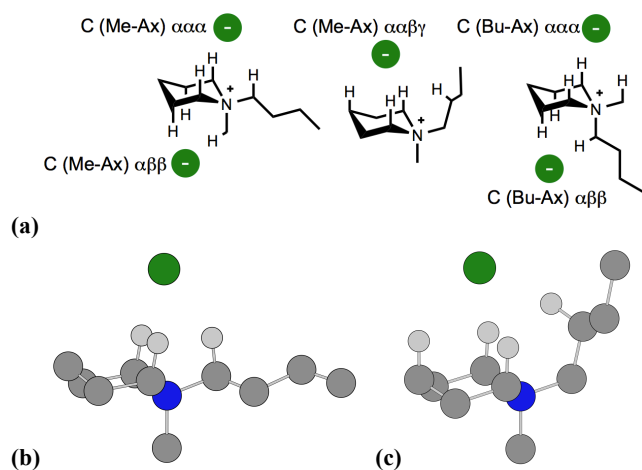
Fig. 3 (a) Primary cation-anion interactions for chair conformers of [\text{C}_4\text{C}_1\text{pip}]\text{Cl} , 2 . Structures of the: (b) 'C (Me-Ax) \alpha\alpha\alpha 1', and; (c) 'C (Me-Ax) \alpha\alpha\beta\gamma ' ion pair conformers of 2 , showing primary H-bond interactions. All other hydrogen atoms are omitted, for clarity.
