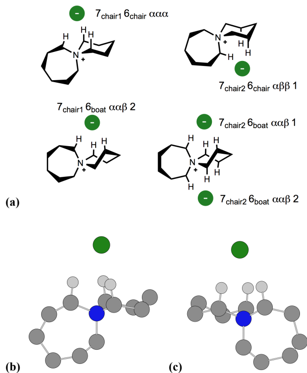
Fig. 4 (a) Diagram representing primary cation-anion interactions for [7+6]Cl, 8 . Structures of the low-energy (b) '7 chair1 6 chair ααα' and (c) '7 chair2 6 chair ααα 1' ion pair conformers of 8 , showing primary H-bond interactions. All other hydrogen atoms are omitted, for clarity.
