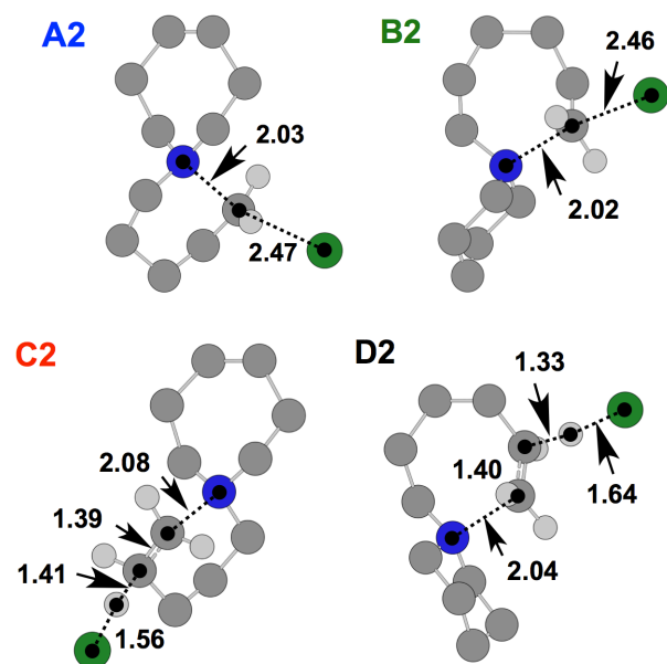
Fig. 12 TS structures for [7+6]Cl, 8 , representing S_N2 (A2, B2) and E2 (C2, D2) mechanisms relative to the lowest energy {}^7\text{chair}_1\text{6chair}_{\alpha\alpha'} ion pair conformer (Fig. 4). Atom distances are in angstroms.
