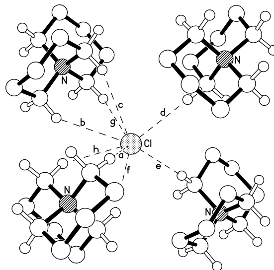
Fig. 2 X-ray crystal structure of [6+6]Cl, 5 , demonstrating apparent C-H...Cl hydrogen-bonding interactions between chloride and neighbouring azoniaspiro cations (only α-H atoms are shown, for clarity).
