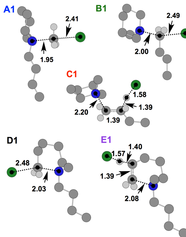
Fig. 11 TS structures for [C 4 C 1 pip]Cl, 2 , representing S N 2 (A1, B1, D1) and E2 (C1, E1) mechanisms. Atom distances are in angstroms.
