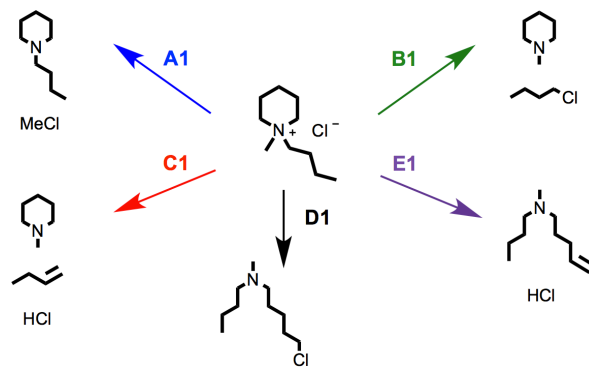
Fig. 7 Proposed S_N2 (A1, B1 and D1) and E2 Hofmann elimination (C1 and E1) thermal decomposition pathways for [C_4C_1pip]Cl , 2 .
