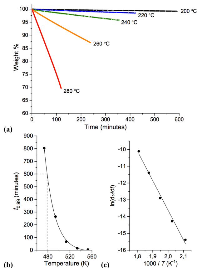
Fig. 6 Determination of the long-term thermal stability of [7+6]\text{Cl} , 8 : (a) Isothermal TGA thermographs; (b) Exponential fit of T (K) vs. t_{0.99} (mins) to determine T_{0.01/10} ; (c) Determination of E_a and A .
