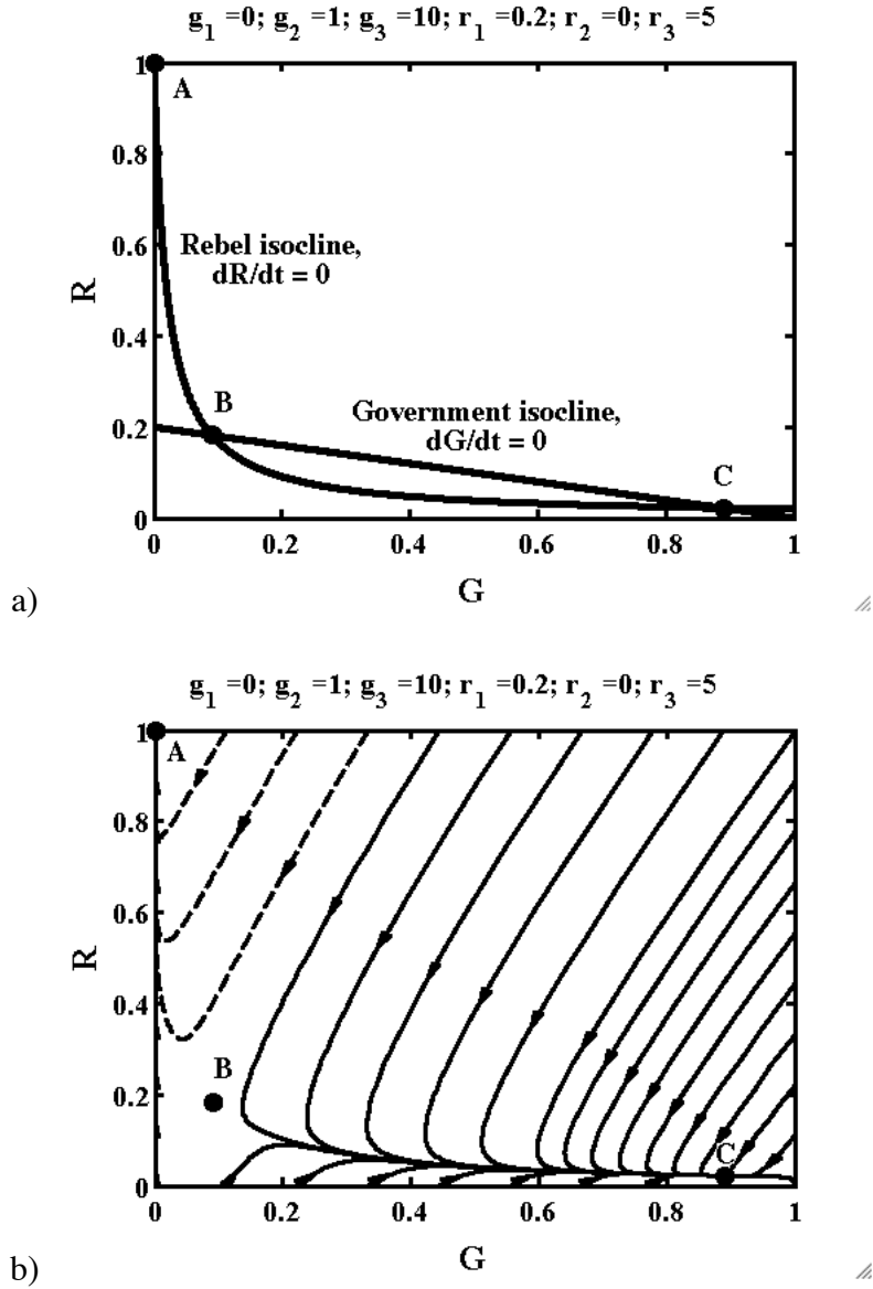
Figure 2. a) Example null isoclines and equilibrium states and b) phase portraits for a government in power, with minor unrest.
