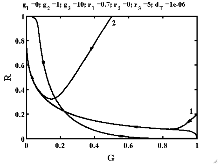
Figure 4. Phase portrait for a cycle of revolutions following from two different initial conditions.
