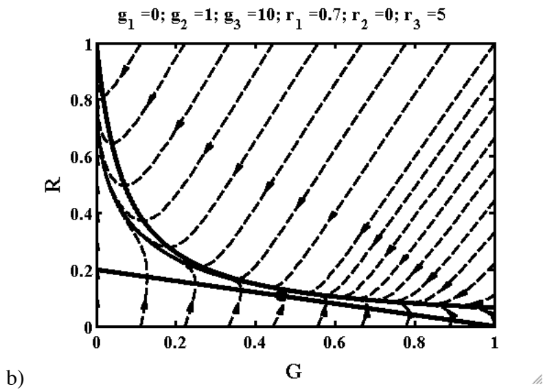
Figure 3. a) Example null isoclines (thick, full lines), equilibrium states (points) and phase portraits (thin, full and dashed lines) for a government initially in power, with a) major unrest and b) rebels gaining power.
