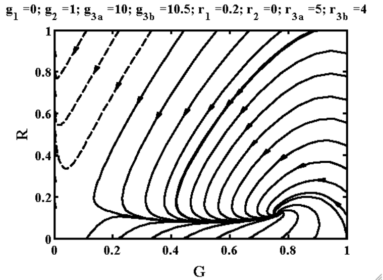
Figure 5. Phase portrait for government in power, but with government and rebels both playing a reactive strategy depending on G.
