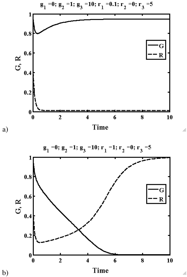
Figure 1. Example time-variation of government (full line) and rebel (dashed line) forces, with a) government and b) rebels winning.
