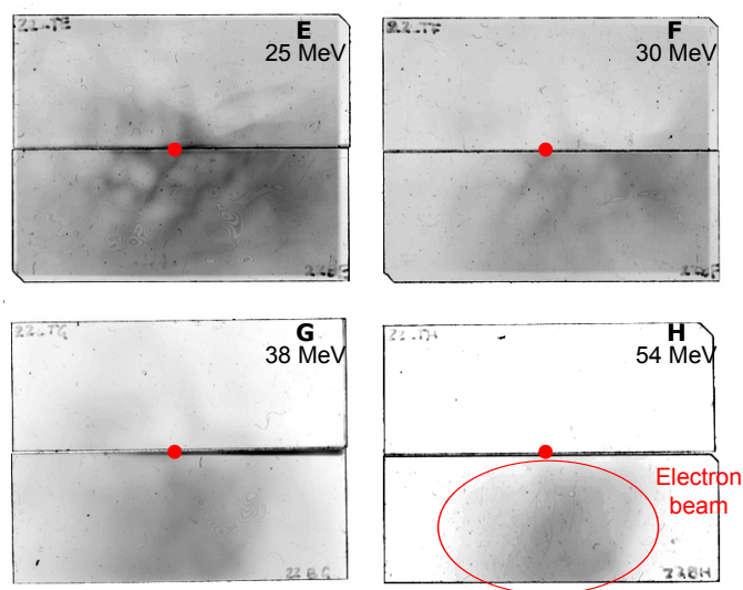
Figure 5. Supplemental Data Figure 5: Red channel from RCF layers at the rear of the stack for a shot with d_0=5 nm DLC, CP (same shot as fig. 2a and supplemental figure 1), showing inferred electron beam at the rear of the stack.
