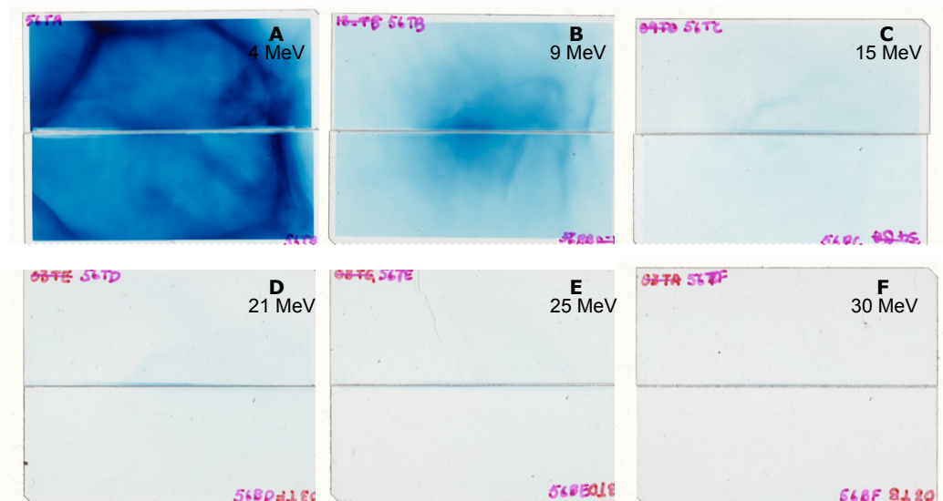
Figure 3. Supplemental Data Figure 3: Unprocessed scans for full RCF stack for 20 nm DLC, CP (fig. 2c in text)
