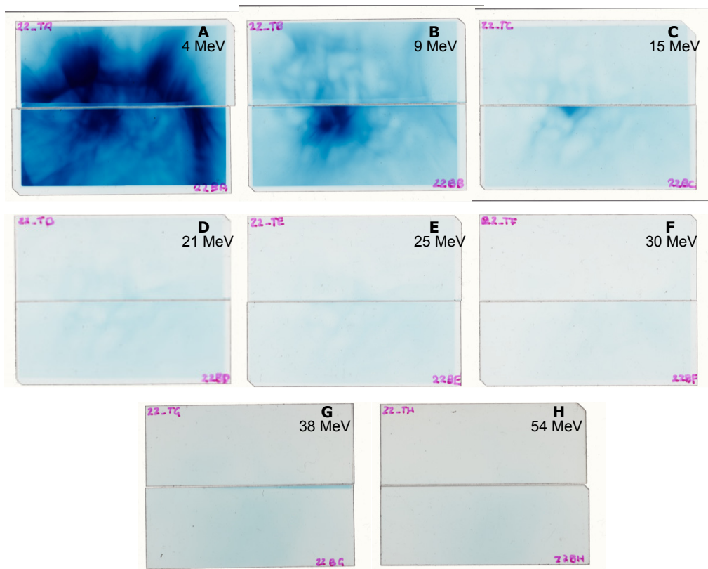
Figure 1. Supplemental Data Figure 1: Unprocessed scans for full RCF stack for 5 nm DLC, CP (fig. 2a in text)
