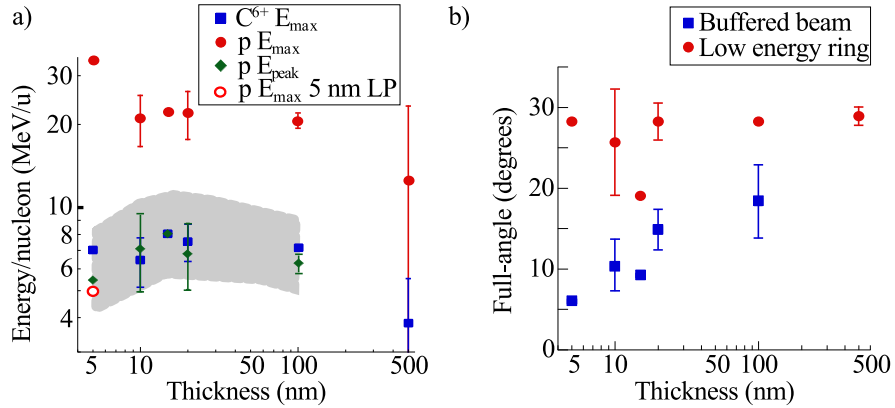
Figure 4. As a function of d_0 : a) maximum energy per nucleon for H^+ (filled red circles, with empty red circle for 5 nm LP) and C^{6+} (blue squares) and energy of H^+ peak (green diamonds) with FWHM energy spread shaded grey; b) divergence of central beam (blue squares, at E = 9 MeV) and low energy ring (red circles, at E = 4 MeV). Vertical bars are the standard deviation of multiple shots.
