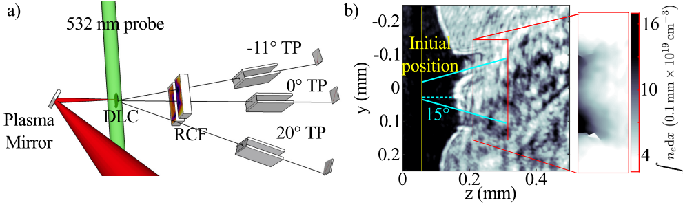
Figure 1. a) Experimental set-up. b) Probe shadowgraphy at t = 250 ps after the interaction together with phase map, in units of the line density integral, from simultaneous interferometry (red box) for d_0 = 100 nm, LP. The yellow line indicates the initial position of the rear surface measured before the shot.
