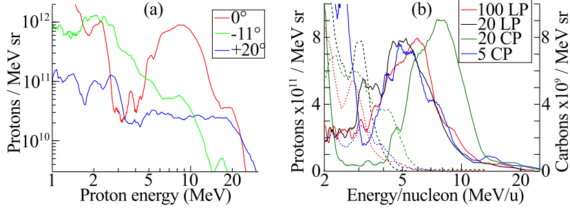
Figure 3. a) H^+ spectra from all TPs from CP, 20 nm target (fig. 2c) on a logarithmic scale. b) H^+ (solid) and C^{6+} ion (dashed) spectra on 0^\circ TP for different polarisations/thickness (in nm) with a linear ion number scale. The 5 nm (CP) corresponds to shot in fig. 2a and the 20 nm (CP) corresponds to fig. 2c.
