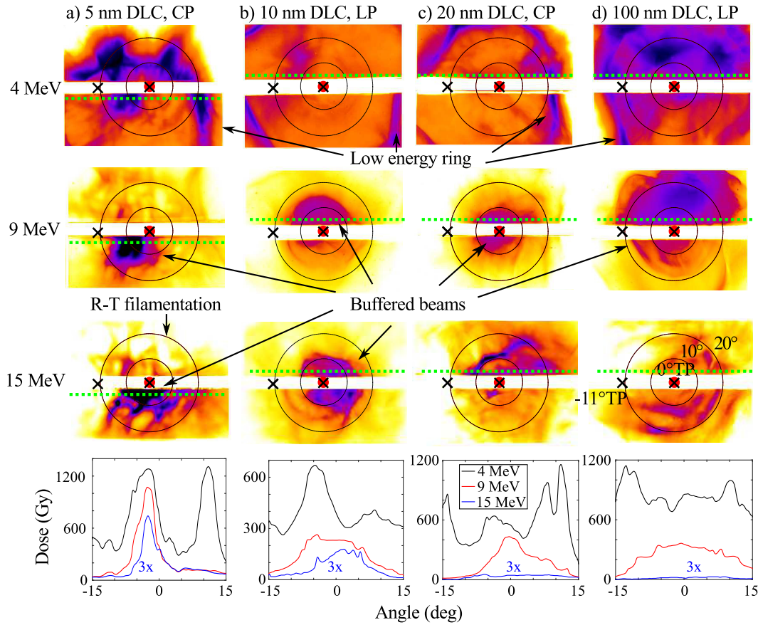
Figure 2. a-d) Proton beam profiles from d_0 = 5, 10, 20, 100 nm using CP, LP, CP, LP respectively at 4, 9, 15 MeV. Red dot represents laser-axis, and black rings are at 10, 20° full-cone angle. The 0, -11° TP are indicated with black crosses. (20° TP is off the right edge). All films are contrast enhanced, and dark colour represents higher dose. Dose line outs from the dotted green lines for each target thickness are given in the bottom row. The E = 15 MeV line out has been multiplied by 3.
