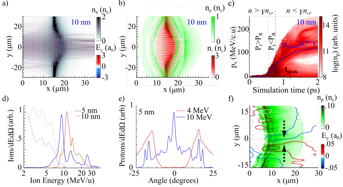
Figure 5. From simulation: a) charge density of electrons and overlaid transverse electric field E_y showing target transparency, and b) charge density of C^{6+} (red) and protons (green) near the peak of pulse, t_{peak} , for d_0 = 10 nm; c) Evolution of p_x for protons on-axis, with p_{x,max} for C overlaid (blue line) for d_0 = 10 nm; vertical dashed (dotted) lines indicate different density (pressure) regimes; d) spectra of protons (solid) and C^{6+} (dotted) witnessed in \approx 1 msr on-axis for d_0 = 5, 10 nm; e) angular proton distribution at 4 and 10 MeV for a 5 nm target; f) n_p at t_{peak} + 200 fs with overlaid electrostatic E_y contours for d_0 = 5 nm.
