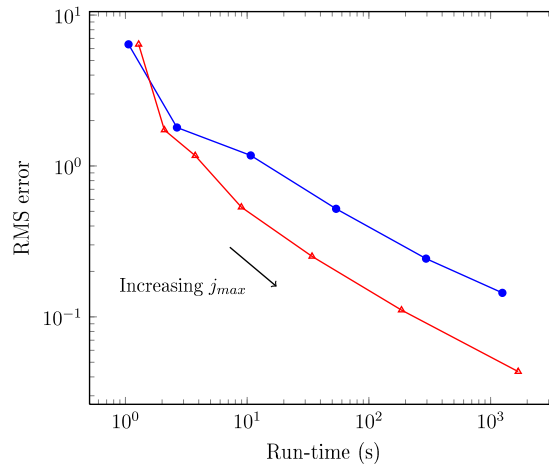
Fig. 9. Depth induced refraction. Convergence tests for uniform P_0 with \{16, 32, 64, 128, 256, 400\} angles \bullet and HW_{3,j} , j_{\max} \in \{4, 5, 6, 7, 8, 9, 10\} , adaptive discretisations for a tolerance \tau = 10^{-1} \blacktriangle . The HW_{3,j} points correspond to the results after the adaptive algorithm converges.
