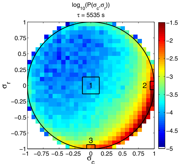
Figure 3. Joint probability distribution of \sigma_c and \sigma_r at time lag \tau = 5535 s for the entire seven day analysis interval.
