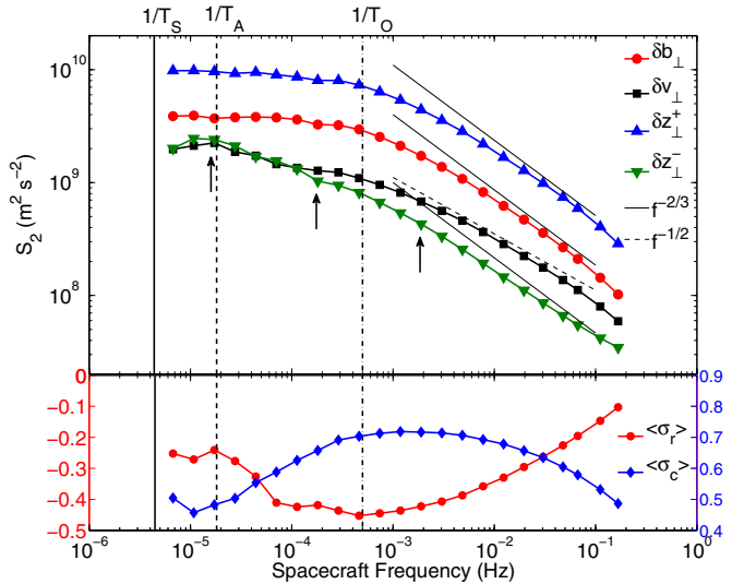
Figure 2. Top panel: structure functions of the vector fields are shown plotted against spacecraft frequency ( f = 1/\tau ). Bottom panel: normalized cross helicity and residual energy (Equations (10) and (11)) averaged over the entire duration of the fast stream. The arrows indicate the lags \tau used in Figure 5, with the middle arrow also indicating the scale used in Figure 3.
