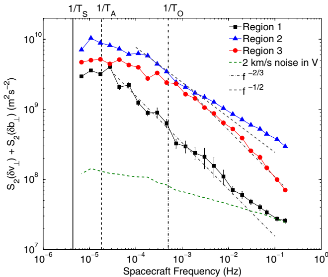
Figure 4. Sum of the velocity and magnetic-field structure functions in three regions of the \sigma_c , \sigma_r plane: Region 1, which contains balanced, equipartitioned fluctuations; Region 2, which contains very pure anti-Sunward Alfvénic fluctuations; and Region 3, which contains very pure magnetic fluctuations. (A color version of this figure is available in the online journal.)
