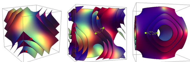
Figure 1. The minimal surfaces that the three lipid inverse bicontinuous cubic phases are based on. From left to right: diamond (Pn3m), gyroid (Ia3d) and primitive (Im3m).
