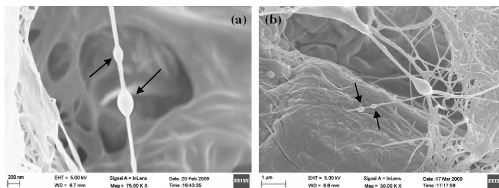
Fig. 2. Typical examples of the SEM images showing PLLA melt droplets on BC nanofibre: (a) neat BC and (b) C 12 -BC.
