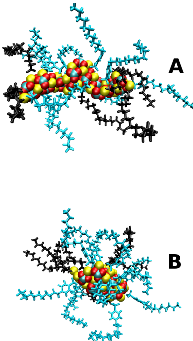
Figure 2: Simulation snapshots of the sulphate-based nanoparticle. A) Stearate added during self-assembly process, PI. B) Stearate added post self-assembly, PII. Calcium ions are shown in yellow, and cyan and red indicate the carbon and oxygen atoms of the carbonate ions, respectively. The sulphate surfactant is shown in cyan, with the stearate co-surfactant shown in black.
