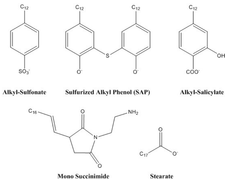
Figure 1: The five surfactant and dispersant types used in this study.
