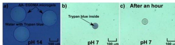
Figure 8. Hydrophilic Trypan Blue encapsulation in, and release from, 50:4 AA-EGDMA microgels. (a) Encapsulation of the dye in pH 14 solution via diffusion. (b) Microgels containing the Trypan Blue immediately after their introduction into a pH 7 environment, and (c) after an hour of dye release at pH 7.
