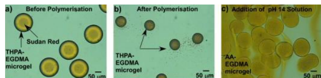
Figure 6. (a) 50:4 THPA-EGDMA microgels with hydrophobic Sudan I dye encapsulated during droplet generation. (b) 50:4 THPA-EGDMA microgels after polymerisation (pH = 7). (c) Sudan I dye release from 50:4 AA-EGDMA microgels in pH 14 solution.
