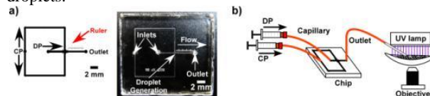
Figure 2: (a) Layout and photograph of the flow focusing chip employed for microgel precursor droplet formation. The design featured a central channel for the oil based DP, containing the reagents, and outer channels for the CP, which merged into a 5 mm long outlet channel. (b) Experimental setup for on-chip droplet generation and collection of the droplets onto a slide or dish for UV initiated photopolymerisation.
