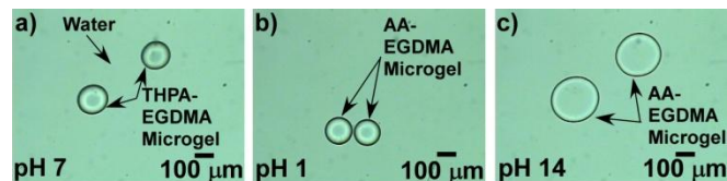
Figure 4. THPA-EGDMA (50:4 molar ratio) microgels (a) before hydrolysis at pH 7, (b) after hydrolysis (forming AA-EGDMA microgels) at pH 1, and (c) at pH 14.
