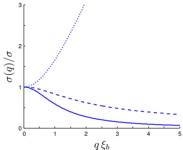
FIG. 1: Comparison of different wavevector dependent surface tensions \sigma(q) : the effective tension \sigma_{\text{eff}}(q) given by eq. (28) as defined from the excess contribution to the total structure factor (dotted line), \sigma_{cc}(q) given by eq. (54) as defined using the crossing criterion (dashed line), and the result from the floating point definition of the interface \sigma_G(q) , eq. (74), (continuous line).
