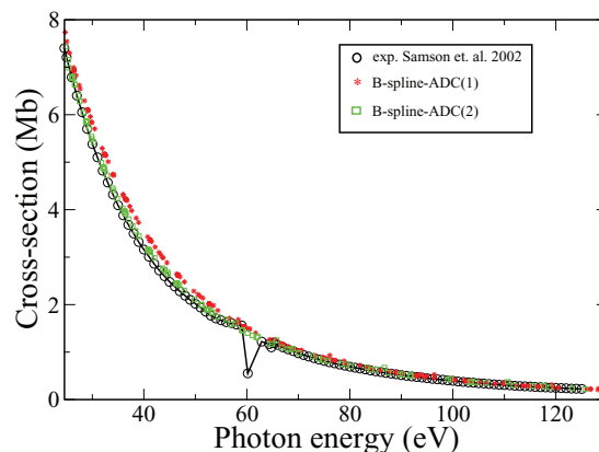
FIG. 3. Total photoionization cross-section of He atom. Circles – experimental result of Ref. 32, stars – B-spline-ADC(1) result, from Stieltjes order 5 to 34; squares – B-spline-ADC(2)-Lanczos-Stieltjes cross-section, using the Stieltjes orders 5–34. Basis set 2 was employed (see Table I). With this basis set, the ADC(1) and ADC(2) matrices for He have the dimensions of 88 \times 88 and 96\,500 \times 96\,500 , respectively. The ADC(2) results was obtained using BL pseudospectrum of 3960 eigenvalues and eigenvectors.
