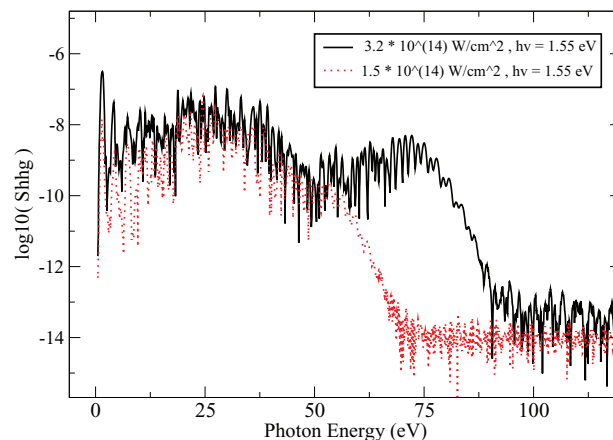
FIG. 14. ADC(1) high harmonics generation emission spectrum of Ar atom interacting with an IR field. The red and black curves refer to the 1.5 \times 10^{14} W/cm 2 and 3.2 \times 10^{14} W/cm 2 values for the IR peak intensity, respectively. The time duration of the IR laser pulse used is about 21 fs and the frequency is 800 nm.
