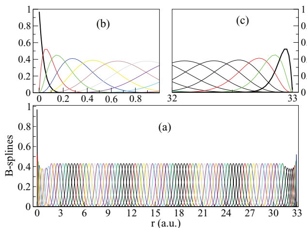
FIG. 1. (a) graphical representation of B-spline basis Set 3, with R_{\max} = 33 a.u.; the knot sequence is linear and the total number of B-spline functions is 97. (b) magnification of the B-spline functions in the radial region close to the origin. (c) magnification of the B-spline functions in the radial region close to the box boundary.
