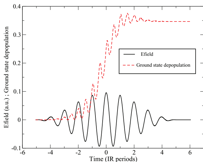
FIG. 13. Time dependent IR electric field and ground state depopulation of Ar atom. The IR peak intensity is 3.2 \times 10^{14} W/cm 2 .
