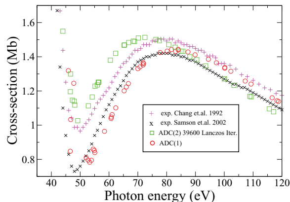
FIG. 7. Total photoionization cross-section of Ar atom. Crosses – experimental result of Ref. 32, pluses – experimental result of Ref. 33, circles – B-spline-ADC(1) result, Stieltjes orders 25–34; squares – B-spline-ADC(2)-Lanczos-Stieltjes cross-section, Stieltjes orders 25–34. The BL pseudospectrum for which the cross-sections convergence is obtained is 30 000.
