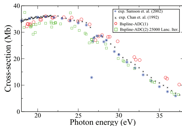
FIG. 6. Total photoionization cross-section of Ar atom. Stars – experimental result of Ref. 32, crosses – experimental result of Ref. 33, circles – B-spline-ADC(1) result, Stieltjes orders 5–18; squares – B-spline-ADC(2)-Lanczos-Stieltjes cross-section, Stieltjes orders 5–18, obtained using BL pseudospectrum of 10 000 eigenvalues and eigenvectors. Basis set 1 was employed (see Table I). With this basis and excitation restrictions, the ADC(1) and ADC(2) matrices have dimension of 602 \times 602 and 396\,541 \times 396\,541 , while the size of the BL pseudospectrum for which the cross-sections convergence is obtained is 10 000.
