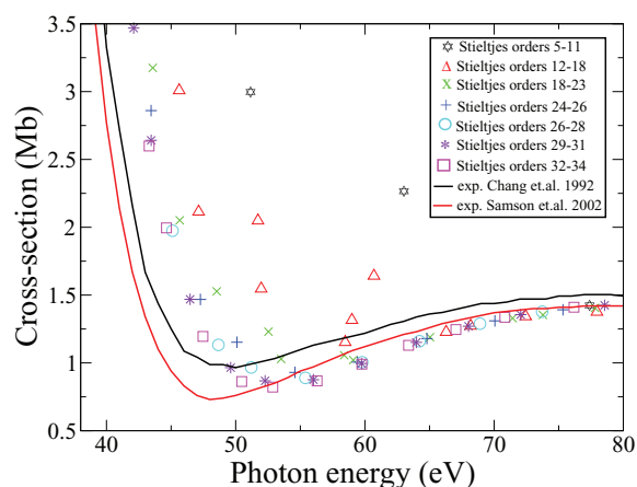
FIG. 9. Total photoionization cross-section of Ar atom in the Cooper minimum energy region. Convergence with respect to the Stieltjes order n is shown for a B-spline ADC(1) calculation done with B-spline set 3. Different symbols represent different orders as indicated in the legend. Full red line – experimental result of Ref. 32, full black line – experimental result of Ref. 33.
