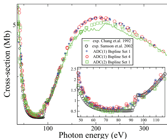
FIG. 11. Total photoionization cross-section of Kr atom. Circles – experimental result of Ref. 32, full green line – experimental result of Ref. 33; stars – B-spline-ADC(1) result using B-spline Set 1, from Stieltjes orders 5 to 34; circles – B-spline-ADC(1) result using B-spline Set 4, from Stieltjes orders 5 to 34; squares – B-spline-ADC(2)-Lanczos-Stieltjes cross-section, from Stieltjes orders 18 to 34, obtained using BL pseudospectrum of 30 000 eigenvalues and eigenvectors.
