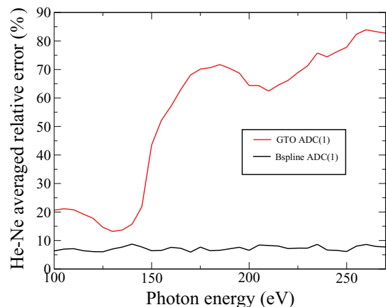
FIG. 5. Relative deviations of the calculated ADC-Stieltjes photoionization cross-sections, averaged over Ne and He atoms, from the experimental result, as a function of the energy in the high energy range, i.e., between 100 eV and 250 eV. Black full line – B-spline-ADC(1)-Stieltjes result, red full line – GTO-ADC(1)-Lanczos-Stieltjes result.
