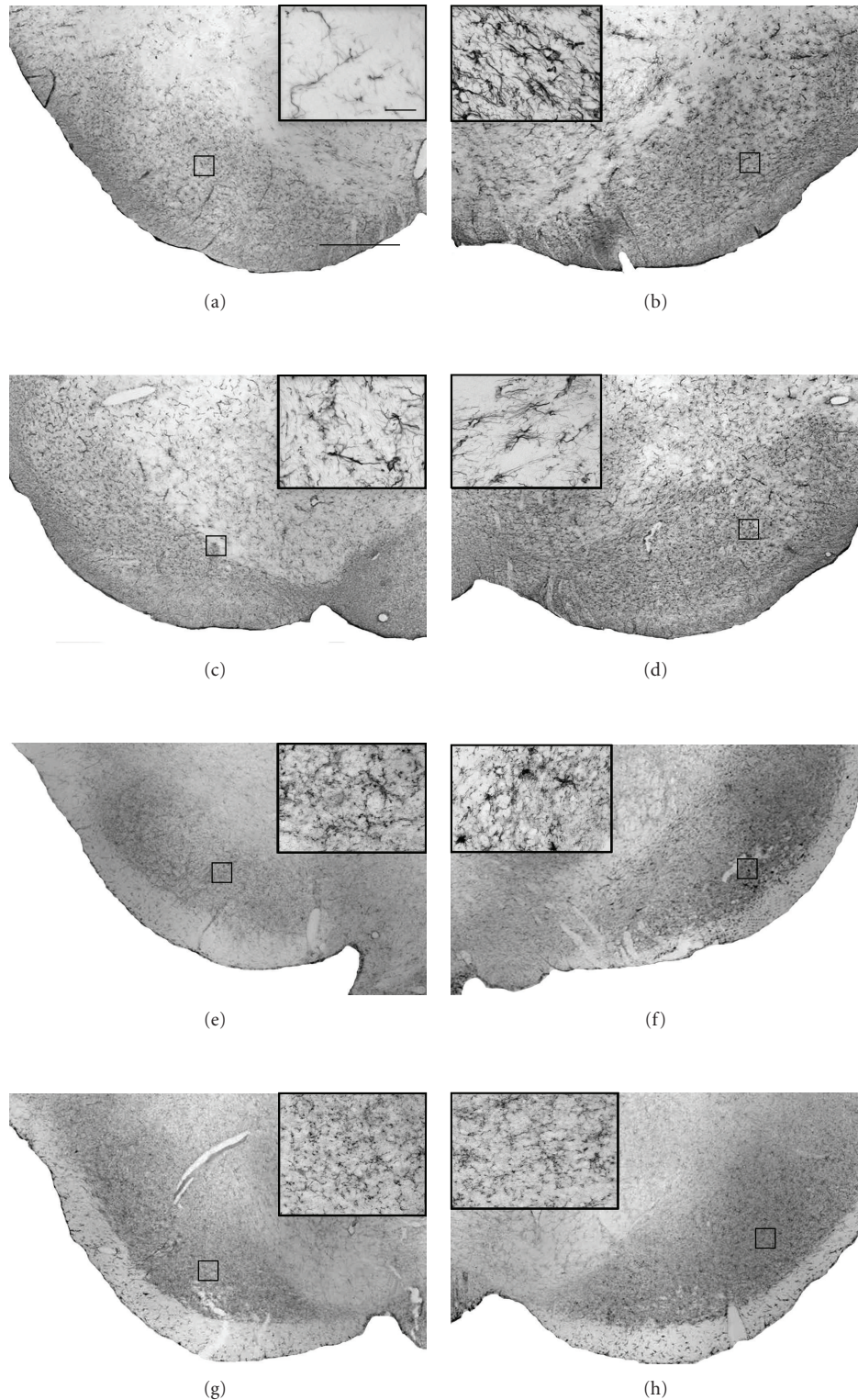
FIGURE 3: Neuroprotection against 6-OHDA toxicity following delayed subchronic intranigral administration of 2 R ,4 R -APDC is associated with qualitative reductions in inflammatory markers. Representative photomicrographs ( \times 40 ) of DAB/oxidase staining for GFAP (astrocytosis) and OX-42 (microgliosis) in the SNc from each treatment group (scale bar 200 \mu\text{m} ). Panels (a)–(g) show the intensity and distribution of GFAP+ and OX-42+ cells in the contralateral control SN of vehicle (a), (c) and (e), (g) 2 R ,4 R -APDC (10 nmol)-injected animals. Panels (b)–(h) show the intensity and distribution of GFAP+ and OX-42+ cells in the Lesioned SNc of vehicle (b), (d) and (e), (g) 2 R ,4 R -APDC (10 nmol)-injected animals. (Insets (a)–(h)), \times 60 , enlargements of outlined areas (scale bar 10 \mu\text{m} ). Note the apparent reduction in intensity of GFAP+ and OX-42+ staining in 2 R ,4 R -APDC-injected animals compared to vehicle-treated animals. Further, 2 R ,4 R -APDC treatment appeared to reduce the number of cells with morphology characteristic for reactive astrocytes or activated microglia in the SNc in comparison to vehicle-treated controls.
