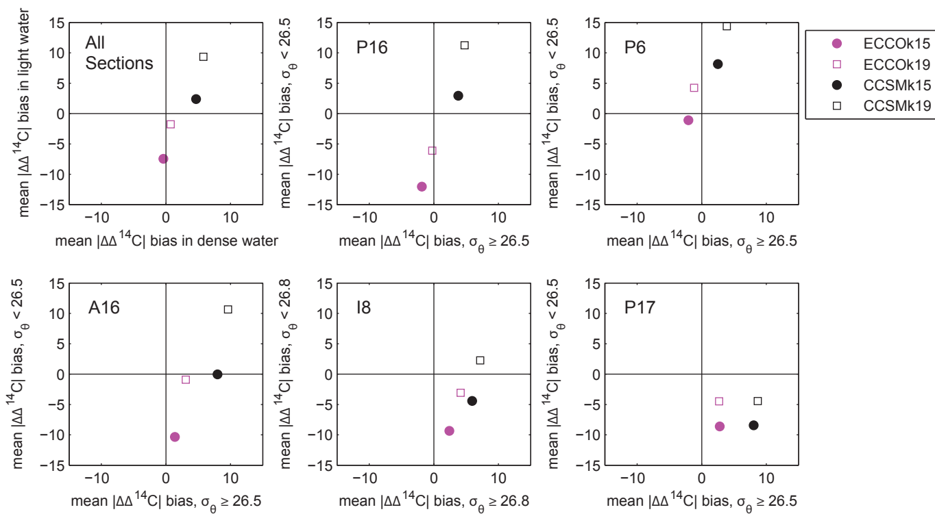
Figure S1. Mean bias in the simulated magnitude of \Delta\Delta^{14}\text{C} for each section. Negative values indicate the magnitude of \Delta\Delta^{14}\text{C} is too small, positive values indicate the magnitude of \Delta\Delta^{14}\text{C} is too large.
