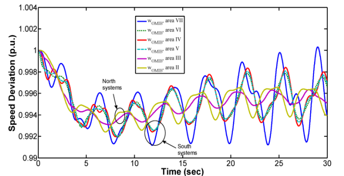
Fig. 12. Time trajectories of the OMIB of the relevant disturbed machine groupings.
