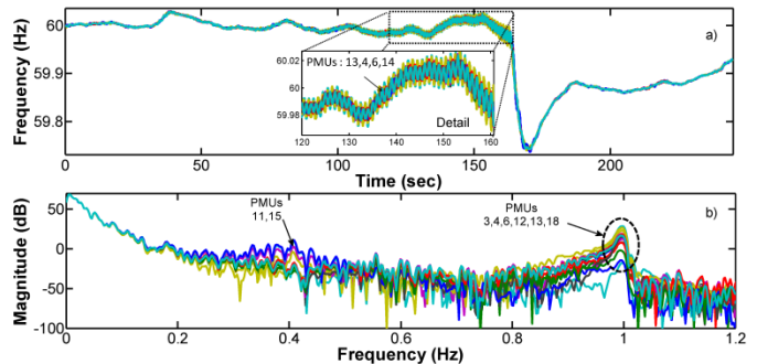
Fig. 15. Time traces of recorded frequency measurements and their associated spectra.
