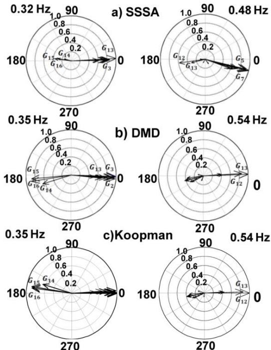
Fig. 7. Mode shape of modes 1 and 2 in Table I showing major coherent groups: a) SSSA, b) DMD, c) Koopman analysis.
