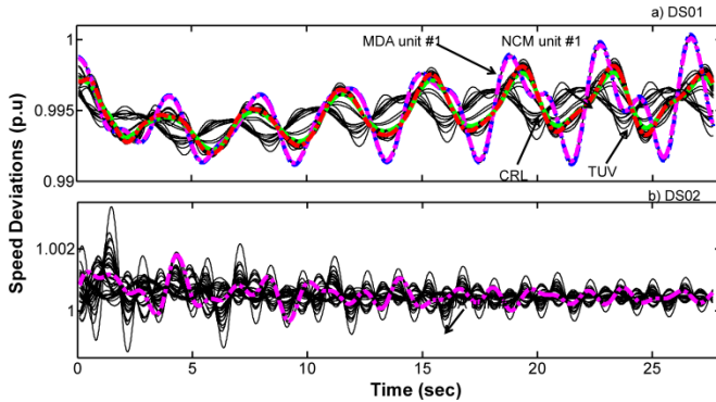
Fig. 9. System dynamic response for scenarios DS01 and DS02.
