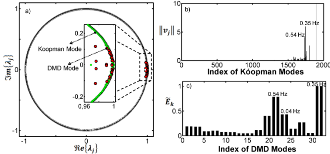
Fig. 4. Empirical Ritz values and their associated norms. a) Empirical Ritz values estimated by Koopman and DMD, b) and c) Norm of dynamic modes and energy amplitudes associated with Koopman and DMD modes.
