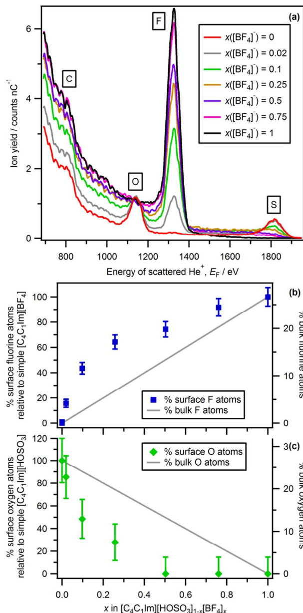
Figure 2. (a) LEIS spectra ( ^4\text{He}^+ , E_0 = 3 keV) for [\text{C}_4\text{C}_1\text{Im}][\text{HOSO}_3]_{1-x}[\text{BF}_4]_x where x([\text{BF}_4]) = 0, 0.02, 0.1, 0.25, 0.5, 0.75 and 1 . (b) % surface fluorine atoms relative to simple [\text{C}_4\text{C}_1\text{Im}][\text{BF}_4] from LEIS data (left axis) and % bulk fluorine atoms (which represents an ideal outer atomic surface composition, right axis) vs. mole fraction x([\text{BF}_4]) for [\text{C}_4\text{C}_1\text{Im}][\text{HOSO}_3]_{1-x}[\text{BF}_4]_x . (c) % surface oxygen atoms relative to simple [\text{C}_4\text{C}_1\text{Im}][\text{HOSO}_3] from LEIS data (left axis) and % bulk oxygen atoms (which represents an ideal outer
