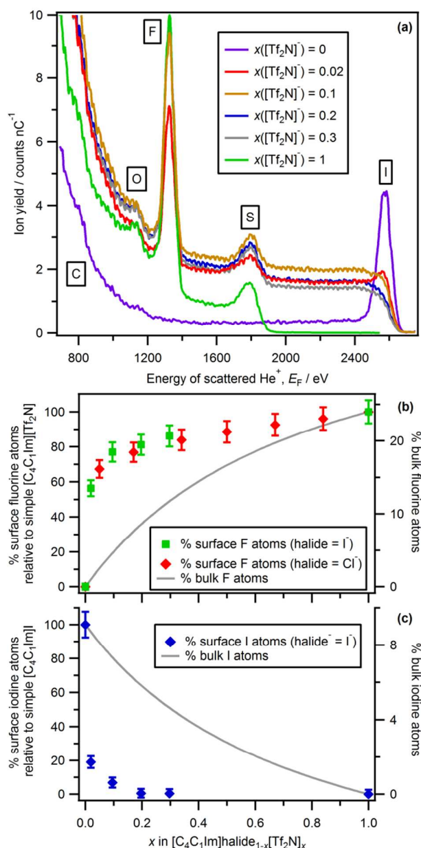
Figure 1. (a) LEIS spectra ( ^4\text{He}^+ , E_0 = 3 keV) for [\text{C}_4\text{C}_1\text{Im}]_{1-x}[\text{Tf}_2\text{N}]_x where x([\text{Tf}_2\text{N}^-]) = 0, 0.02, 0.1, 0.2, 0.3 and 1 . (b) % surface fluorine atoms relative to simple [\text{C}_4\text{C}_1\text{Im}][\text{Tf}_2\text{N}] from LEIS data (left axis) and % bulk fluorine atoms (which represents an ideal outer atomic surface composition, right axis) vs. mole fraction x([\text{Tf}_2\text{N}^-]) for [\text{C}_4\text{C}_1\text{Im}]_{1-x}[\text{Tf}_2\text{N}]_x and [\text{C}_4\text{C}_1\text{Im}]\text{Cl}_{1-x}[\text{Tf}_2\text{N}]_x . (c) % surface iodine atoms relative to simple [\text{C}_4\text{C}_1\text{Im}]\text{I} (left axis) and % bulk iodine atoms (which represents an ideal outer atomic surface composition, right axis) vs. mole fraction x([\text{Tf}_2\text{N}^-]) for [\text{C}_4\text{C}_1\text{Im}]_{1-x}[\text{Tf}_2\text{N}]_x .
