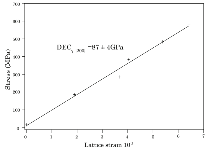
Figure 8: Stress-lattice strain graph showing the \{200\} \gamma' and \gamma in the loading direction for 2Ta #2 at room temperature in the Vulcan experiment. The uncertainties of the \gamma and \gamma' lattice strains are estimated from Igor Pro, which are in the range of 10^{-5} to 10^{-4} .
