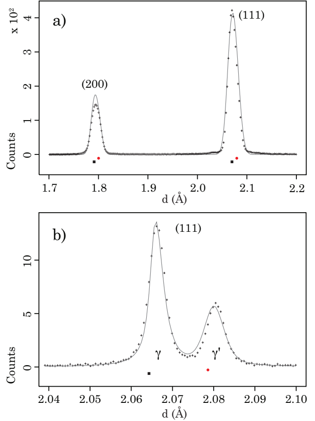
Figure 3: Examples of the fitted diffraction spectra obtained from the 2Ta alloy at RT and zero load. a) by SXRD (I12, Diamond), b) by neutron diffraction (HRPD). Red circle and black square markers correspond to \gamma' and \gamma peaks respectively.
