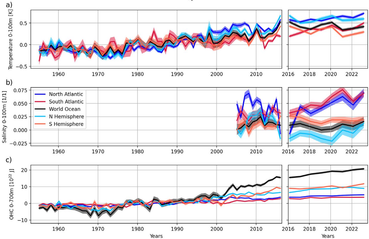
Fig. 3. NCEI data, January–March averages. (a) Ocean temperature anomalies (0–100-m average) 1955–2023. (b) Salinity anomalies (0–100-m average) 2005–23. (c) Ocean heat content anomalies 1955–2023 in the top 700 m. For all panels, the reference period is 1955–2006, and the shading indicates the observational uncertainty. Panels in the right column are a close-up for the years since 2016.
