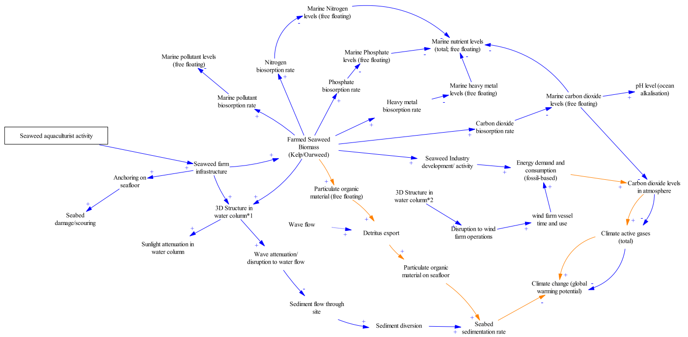
Fig. 6. Standardised and shared cognitive model on the potential impacts to environmental (abiotic) system of the hypothetical scenario of expanding seaweed aquaculture inside Hornsea Wind Farm over the next ten years. -Boxed variable indicates starting node; Arrows show direction of influence between proposed variables (blue for primary and orange for additional/secondary pathways suggested by experts); Dashed lines explain key exogenous variables expressed by participant; plus/minus symbols denote the direction of change i.e. increasing or decreasing, of child nodes. (For interpretation of the references to colour in this figure legend, the reader is referred to the Web version of this article.)
