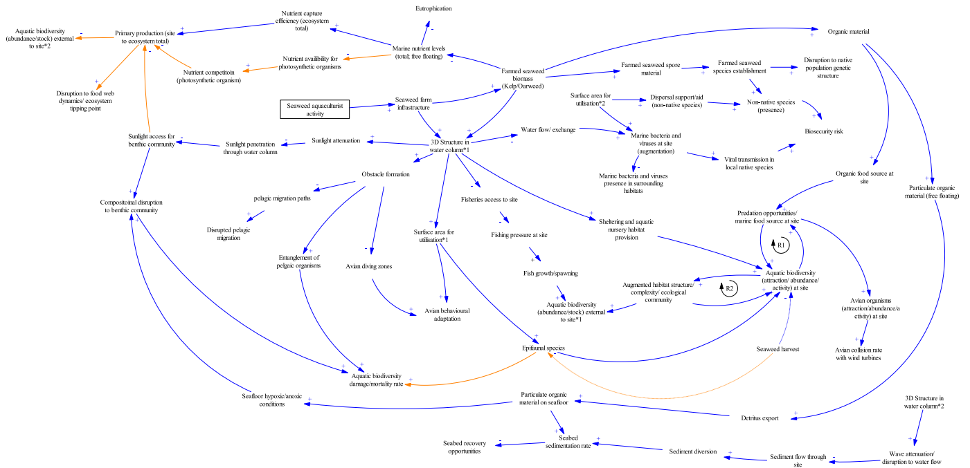
Fig. 7. Standardised and shared cognitive model on the potential impacts to environmental (biotic) system of the hypothetical scenario of expanding seaweed aquaculture inside Hornsea Wind Farm over the next ten years. -Boxed variable indicates starting node; Arrows show direction of influence between proposed variables (blue for primary and orange for additional/secondary pathways suggested by experts); Dashed lines explain key exogenous variables impacting the seaweed farm system; plus/minus symbols denote the direction of change i.e. increasing or decreasing, of child nodes; Rn highlights reinforcing feedback loop; *n indicates secondary or tertiary impacts to/from a node. (For interpretation of the references to colour in this figure legend, the reader is referred to the Web version of this article.)
