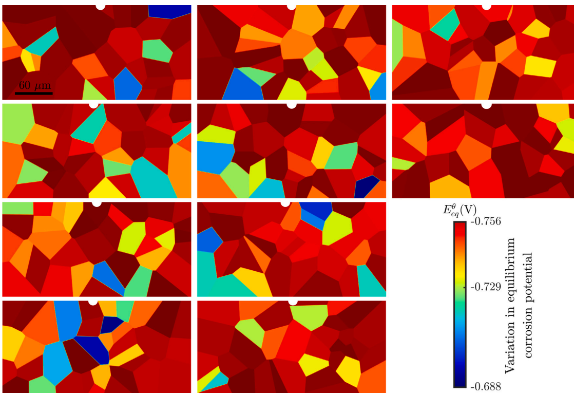
Fig. A.3. Grain morphology distributions for the average grain size of 40 \mu\text{m} . The color bar represents variation in equilibrium corrosion potential with \Delta E^\theta = 10\%E_{eq} (vs. SCE) and applies to all figures. E_{eq} = -0.729 V (vs. SCE) is the macroscopic equilibrium corrosion potential. The width and height of the polycrystalline material are 300 \mu\text{m} and 150 \mu\text{m} , Fig. 8. The surrounding corrosive environment is not shown in these figures.
