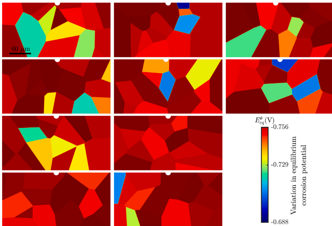
Fig. A.4. Grain morphology distributions for the average grain size of 60 \mu\text{m} . The color bar represents variation in equilibrium corrosion potential with \Delta E^{\theta} = 10\%E_{eq} (vs. SCE) and applies to all figures. E_{eq} = -0.729 V (vs. SCE) is the macroscopic equilibrium corrosion potential. The width and height of the polycrystalline material are 300 \mu\text{m} and 150 \mu\text{m} , Fig. 8. The surrounding corrosive environment is not shown in these figures.
