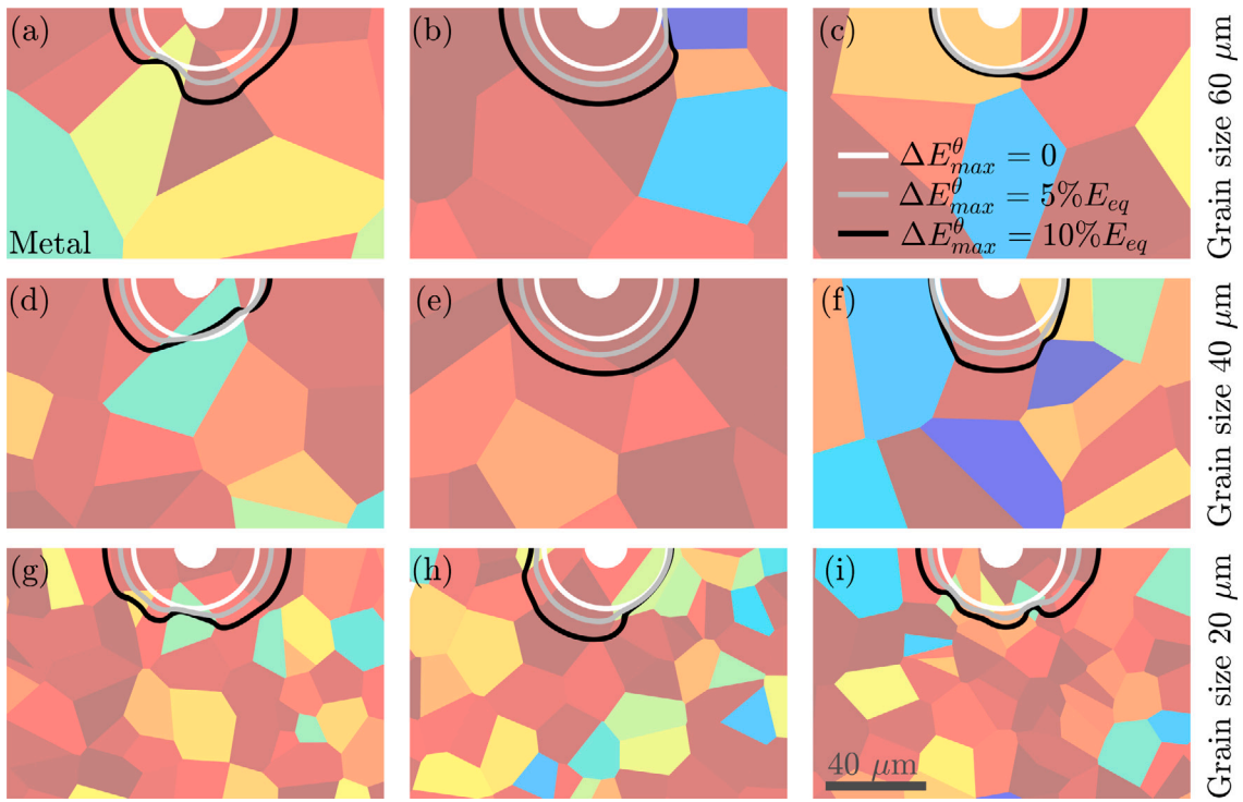
Fig. 9. Evolved pit shapes at the final computational time for activation-controlled corrosion for three representative microstructures with an average grain size of (a–c) 60 μm, (d–f) 40 μm, and (g–i) 20 μm. The black and gray lines represent pit shapes for nonhomogeneous equilibrium corrosion potential with \Delta E_{max}^{\theta} = 10\% E_{eq} and \Delta E_{max}^{\theta} = 5\% E_{eq} variations. The white line stands for pitting corrosion with a uniform corrosion potential. The surrounding environment is not shown in the plots. The scale bar applies to each plot. The color scale for variations in equilibrium corrosion potential is given in Fig. 3.
