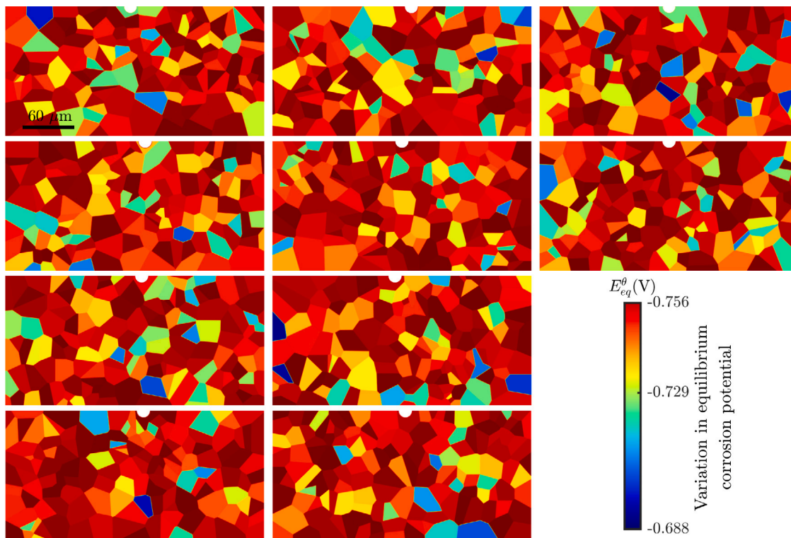
Fig. A.2. Grain morphology distributions for the average grain size of 20 \mu\text{m} . The color bar represents variation in equilibrium corrosion potential with \Delta E^\theta = 10\%E_{eq} (vs. SCE) and applies to all figures. E_{eq} = -0.729 V (vs. SCE) is the macroscopic equilibrium corrosion potential. The width and height of the polycrystalline material are 300 \mu\text{m} and 150 \mu\text{m} , Fig. 8. The surrounding corrosive environment is not shown in these figures.
