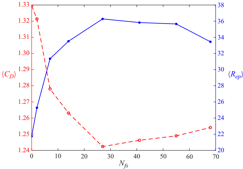
Figure 9. Average drag coefficient ( C_D ) and average episode reward ( R_{ep} ) in PM cases against number history length (numbers of stacked frames) N_{fs} . Here, \langle C_D \rangle is obtained from the asymptotic regime of control, and \langle R_{ep} \rangle is calculated from two episodes after convergence of RL.
