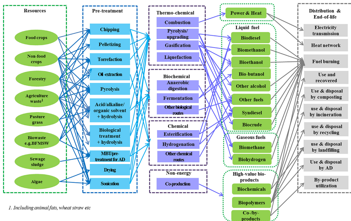
Fig. 7. Pre-treatment and conversion pathways for biorenewable production.
