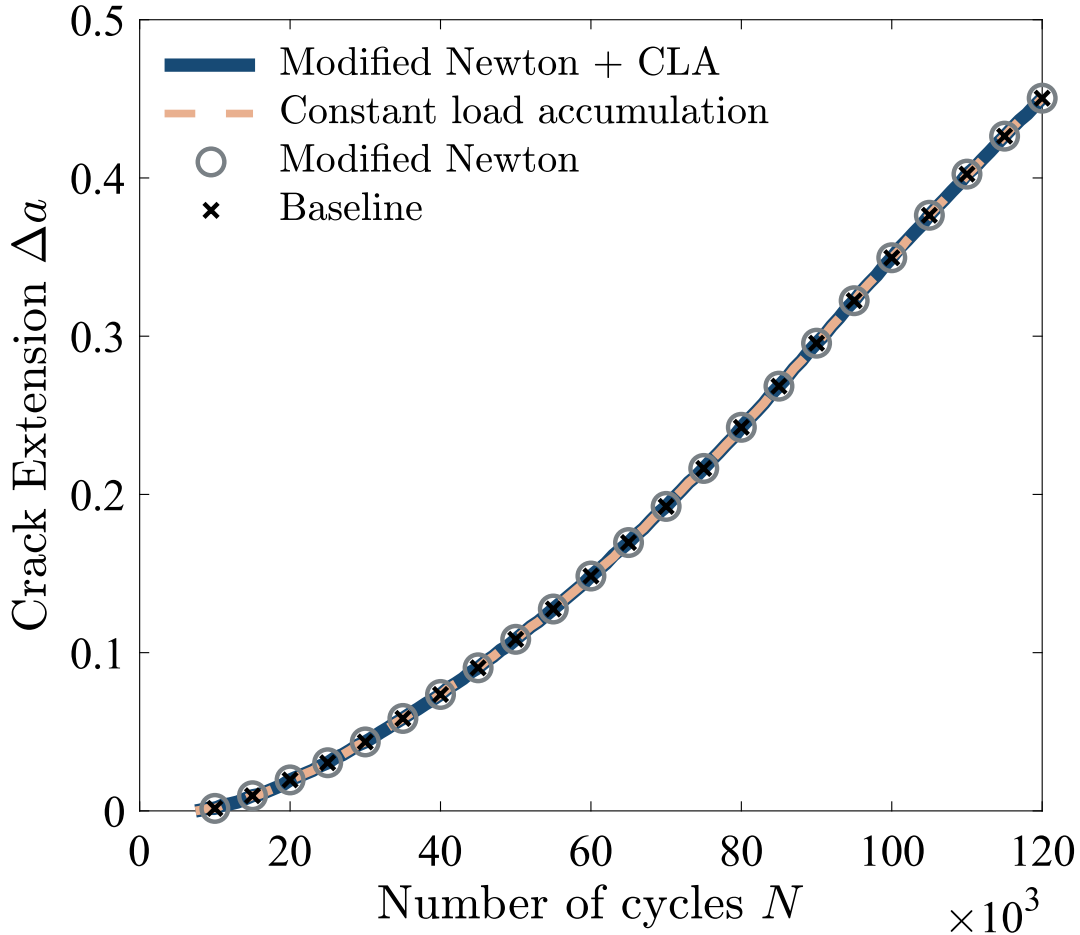
Figure 3: Predictions of crack extension \Delta a versus number of cycles N for the SENT case study. The figure shows results obtained with the reference (baseline) conditions, and the two acceleration scheme presented here (Modified Newton, NM; Constant load accumulation, CLA), independently and in tandem.
