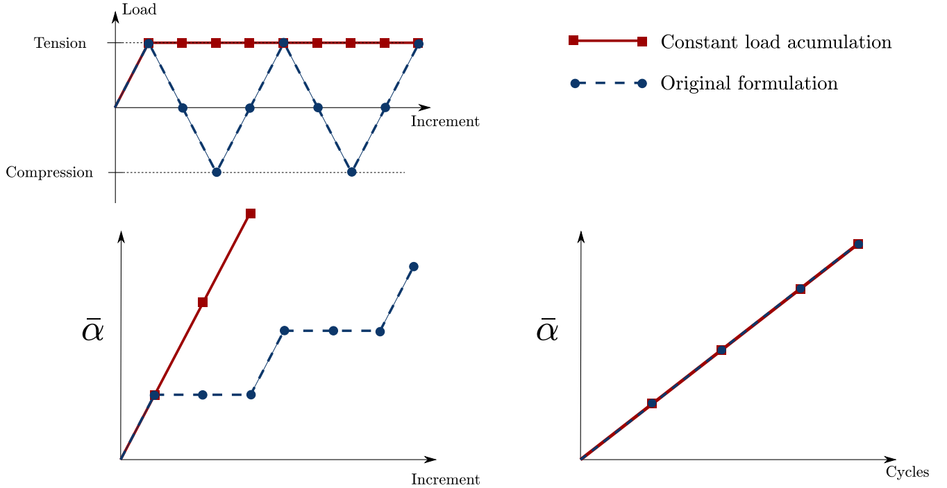
Figure 1: Illustration of loading pattern and fatigue accumulation for the original formulation on the left and the proposed constant load accumulation scheme of the right. As illustrated, the former requires at least four increments per load cycle, while the latter requires only one.
