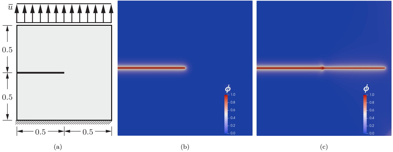
Figure 2: Fatigue crack growth in a Single Edge Notched Tension (SENT): (a) geometry (with dimensions in mm) and boundary conditions, (b) initial crack contour, and (c) final stage of the fatigue crack propagation.
