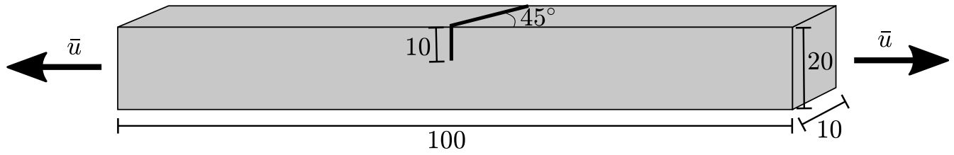
Figure 7: Sketch of the three-dimensional beam undergoing uniaxial tension and containing a tilted edge crack, including the sample dimensions (in mm) and boundary conditions.
