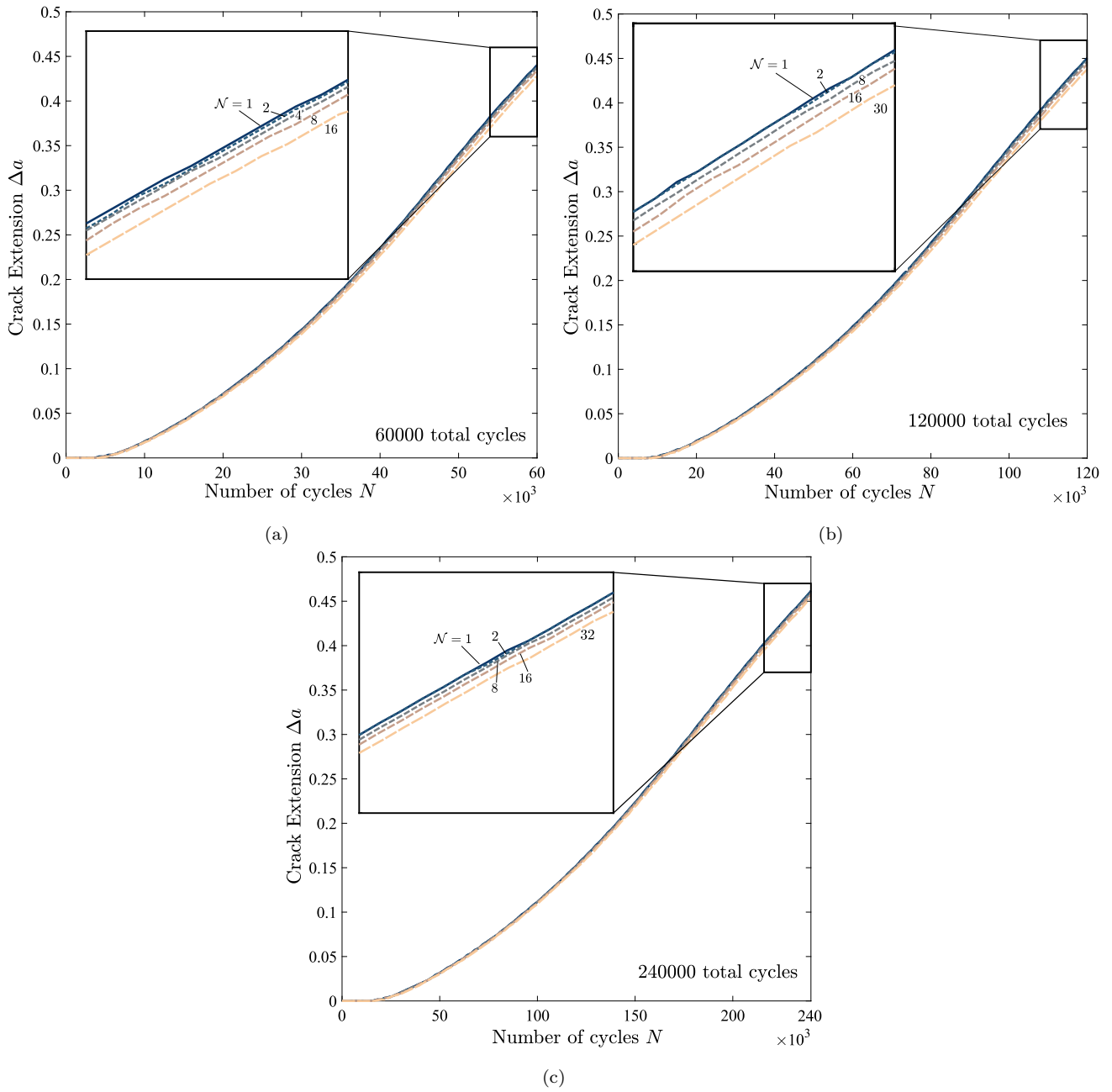
Figure 4: Predictions of crack extension \Delta a versus number of cycles N for the SENT case study considering selected values of \mathcal{N} (number of cycles per increment) and the following characteristic number of cycles: (a) 60,000 cycles, (b) 120,000 cycles, and (c) 240,000 cycles.
