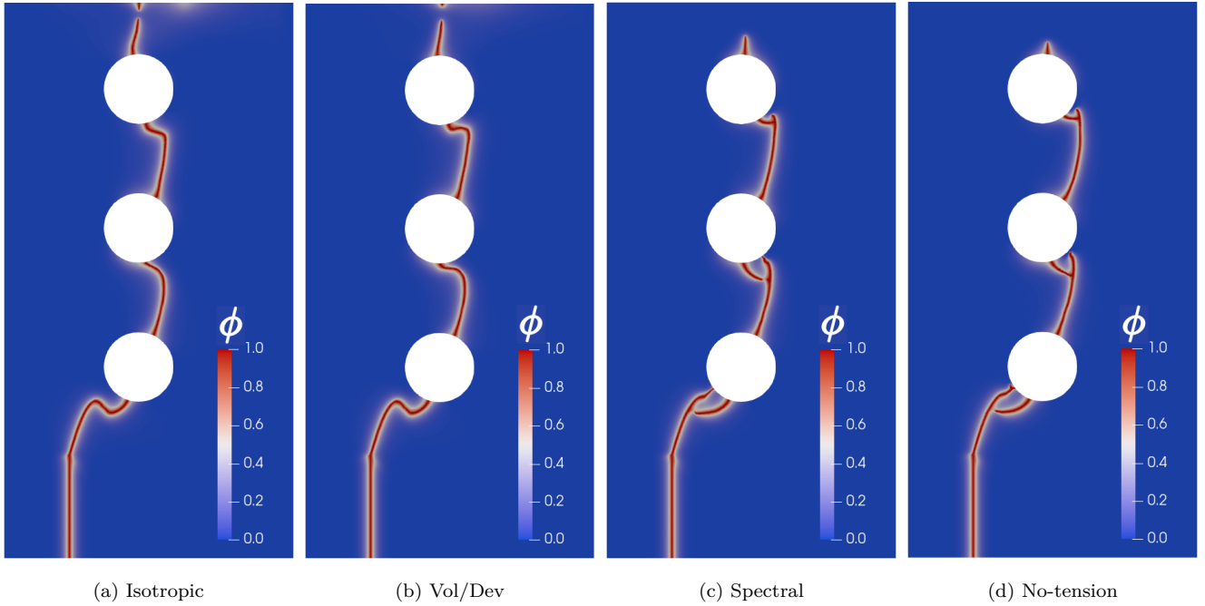
Figure 6: Asymmetric three point bending: Contours of the phase field crack growth after 90,000 fatigue cycles using a) no strain decomposition. b) The volumetric/deviatoric strain decomposition of [53]. c) The spectral decomposition of [54]. d) The no-tension split of [56].
