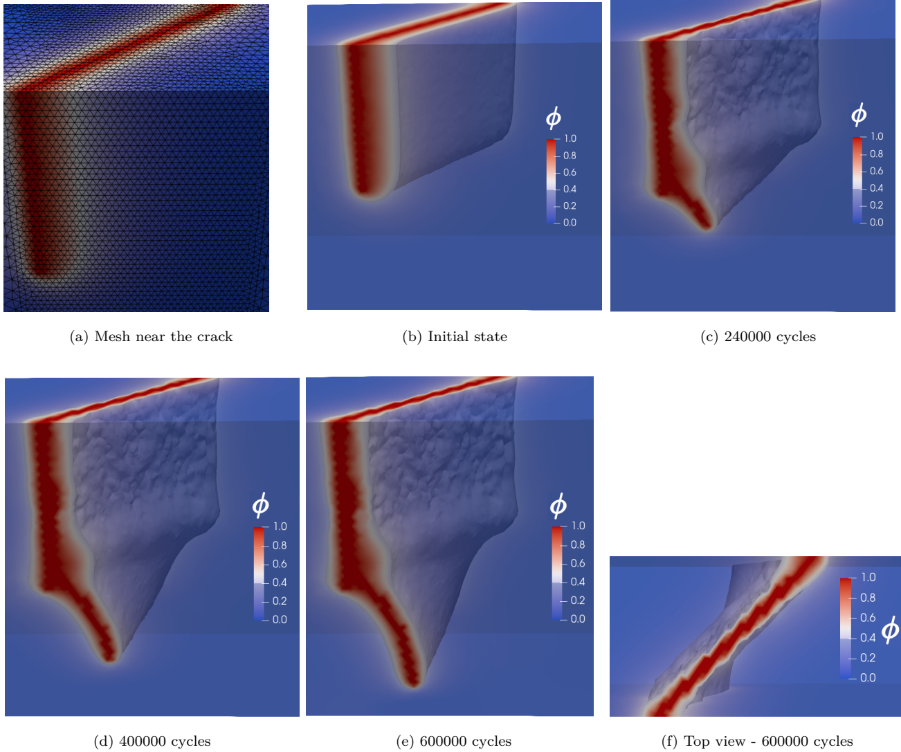
Figure 8: Contours of the 3D tension problem. The crack rotates to be perpendicular to the overall maximal principal stress.
