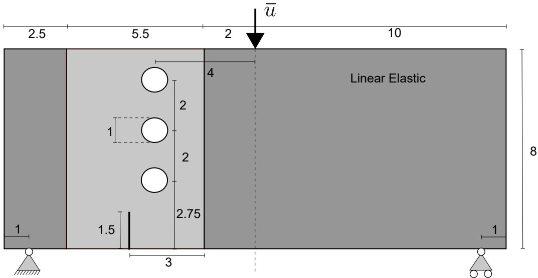
Figure 5: Sketch of the asymmetric three point bending problem, including dimensions (in mm) and boundary conditions. Only the light gray region is subject to fatigue damage.
