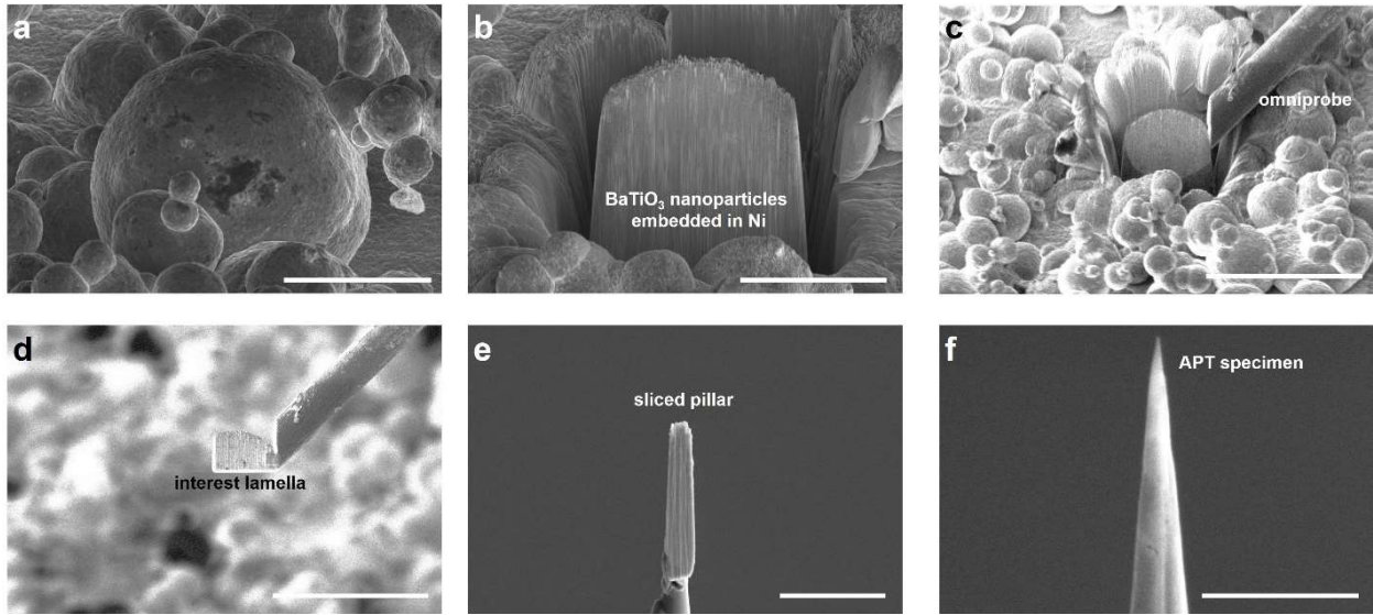
Figure 2. APT specimen preparation for the Ni-coated BaTiO 3 powder sample: (a) 52° tilted SEM image of a selected protrusion region. (b) Trenches were milled 15 μm in depths on the front/back and the left-side of the region of interest with a width of 1 μm. (c) An L-shape horizontal cut was made at the bottom and side of the sample in 52° relative to the ion-beam column, after welding on an omni-probe. (d) The sectioned lamella was lifted-out. (e) Subsequently, the sample was welded with a FIB-Pt deposition on a commercial Si micro-post on only one side where a free cut was done. (f) Thereafter, a free-cut sample was annular milled from the top in decreasing diameters until the apex radius was below 100 nm and the capped Ni layer was removed. The white scale bars are (a,b) 20, (c,d) 50, (e) 10, (f) 1 μm.
