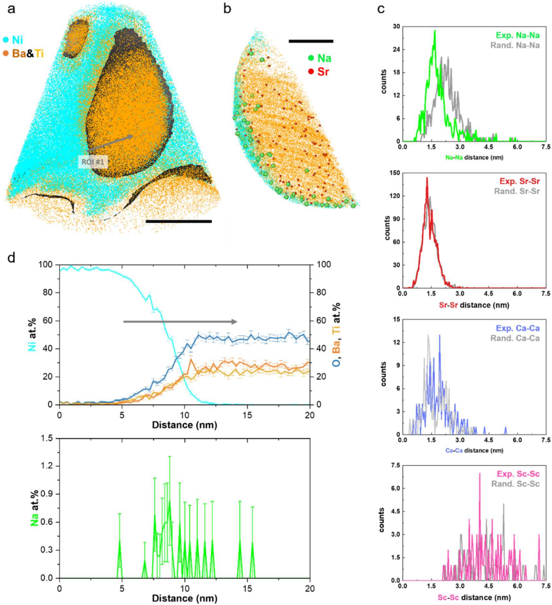
Figure 3. (a) 3D atom map of BaTiO 3 particles embedded in Ni. (b) Distribution of constituent elements (Ba, Ti, Na, Sr) extracted from the atom map. (a,b) scale bars are 20 nm. (c) Nearest-neighbor displacement analyses of Na, Sr, Ca, and Sc elements. (d) 1D compositional analysis along the particle surface. A gray arrow marks the interest profile.
