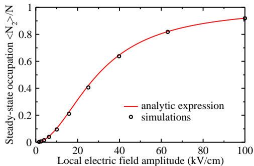
Figure 4. Comparison between simulation results (black circles) and the analytic expression (3.9) for the normalized steady-state occupation density of the upper emission state \langle N_2 \rangle / N of the four-level system (red solid line) when pumping at the absorption resonance \lambda_{0,a} = 680 nm. The parameters of the four-level gain material are given in table 2 and correspond to a saturation field amplitude of E_{\text{sat}} \approx 29.4 kV/cm. (Online version in colour.)
