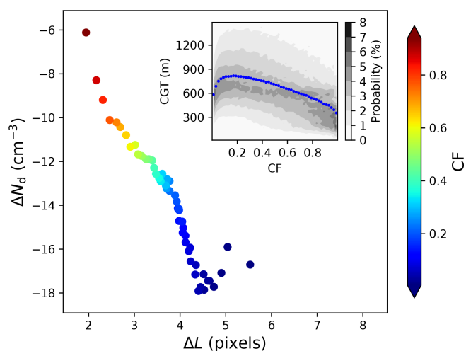
Figure 6. Relationships between \Delta L and \Delta N_d , with the data grouped as a function of CF and each CF bin containing the same number of samples. A joint histogram between CF and CGT is shown in the inner plot; the blue dot shows the median CGT at each CF bin.
