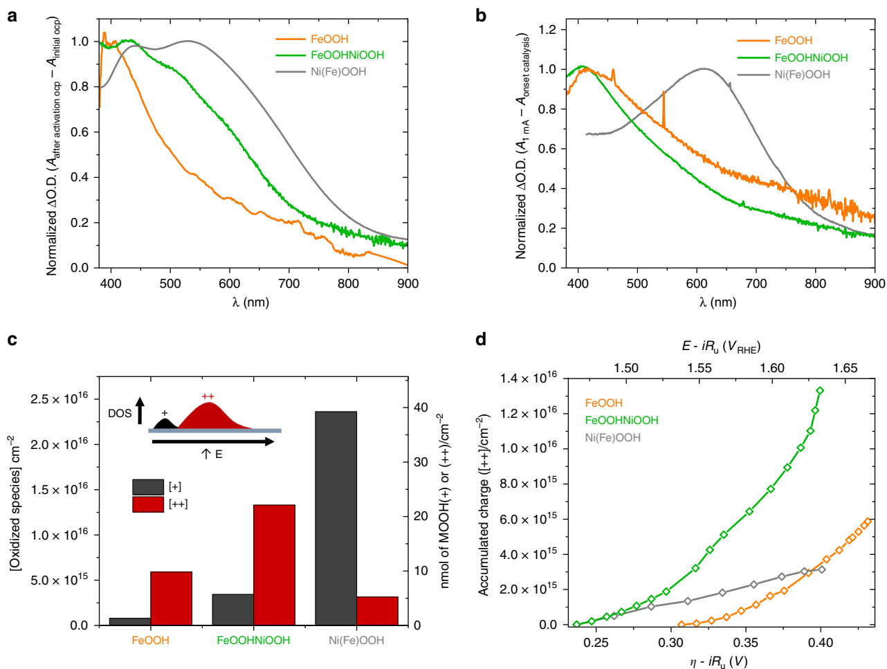
Fig. 2 Accumulated ( + ) and ( ++ ) species for each electrocatalyst. a Normalised \Delta O.D. spectra (to 1 at peak \Delta O.D.) for the first ( 0/+ ), precatalytic, oxidation of FeOOH (orange), FeOOHNiOOH (green) and Ni(Fe)OOH (grey), obtained from the difference between the spectra at open circuit potential (OCP) after and before activation. b Normalised \Delta O.D. spectra for the ( + / ++ ) oxidation wave correlated with water oxidation for FeOOH (orange), FeOOHNiOOH (green) and Ni(Fe)OOH (grey), obtained by subtracting spectra at OCP after activation from the spectra at 1 \text{ mA}/\text{cm}^{-2} of current density. c Concentrations of oxidised \text{MOOH}(+) states generated in the activation process (black) and of \text{MOOH}(++) states generated at a current density of 1 \text{ mA}/\text{cm}^{-2} (red) for each electrocatalyst. Inset: schematic representation of the corresponding densities of states (DOS) for these electrocatalysts. d Accumulated concentrations of \text{MOOH}(++) states vs. the applied overpotential (empty diamonds, solid lines). For both graphs FeOOH (orange), FeOOHNiOOH (green) and Ni(Fe)OOH (grey)
