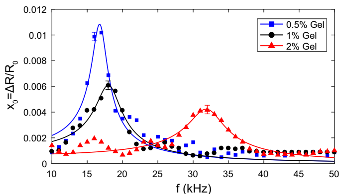
Fig. 4 Resonance curves in 0.5%, 1% and 2% gels respectively. The solid line is a fit of Eq. (10) to the experimental data.
