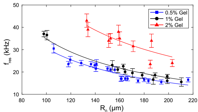
Fig. 5 Summary of experimental data for all bubbles: resonance frequency as a function of bubble radius for each gel concentration. The solid line is a fit to Eq. (9).
