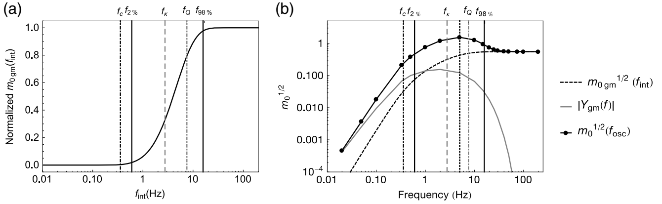
Figure 2. Plot depicting the contribution of Fourier spectral amplitudes, |Y_{gm}(f)| to the response spectral amplitudes at low and high oscillator frequencies. (a) Normalized zeroth-spectral moment m_{0gm} as a function of frequency, f_{int} that is computed as described in equation (9) using |Y_{gm}(f)|^2 . The vertical lines correspond to the source-corner frequency, f_c , f_{2\%} , half-power points related f_k and f_Q , and f_{98\%} . (b) The square root of zeroth-spectral moment m_0^{1/2}(f_{osc}) (thick solid black curve) is considered to represent all the characteristics of the response spectrum y_{max}(f_{osc}) (see Fig. 1c). The gray curve represents |Y_{gm}(f)| corresponding to the input Fourier amplitude spectrum (FAS) (without the SDOF response); and the dashed curve indicates the (square root of) integral of |Y_{gm}(f)|^2 , that is, m_0^{1/2}(f_{int}) . The plots are shown for magnitude M_w 6 at a distance R_{JB} = 20 km; and the same stochastic model parameters as used for Figure 1.
