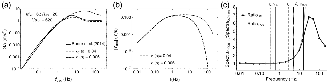
Figure 10. Plots depicting the effect of an adjustment made in the site related attenuation parameter, \kappa_0 on FAS, |Y_{gm}(f)| and its impact on the response spectrum, y_{max}(f_{osc}) . (a) The response spectral ordinates obtained from the model of Boore et al. (2014) along with those obtained from stochastic simulations for \kappa_0 values 0.04 (host) and 0.006 (target) (s). (b) Simulated FAS, |Y_{gm}(f)| for the two \kappa_0 values. (c) The ratios as y_{max,0.006 s}(f_{osc})/y_{max,0.04 s}(f_{osc}) and |Y_{gm,0.006 s}(f)|/|Y_{gm,0.04 s}(f)| for response spectral ordinates and FAS respectively. The vertical lines indicate source-corner frequency f_c (dotted dashed), \kappa_0 related corner frequency f_{\kappa} (dashed gray), and Q related corner frequency f_Q (gray dotted dashed), f_{2\%} and f_{98\%} (solid-black). The dotted vertical line between f_{\kappa} and f_Q corresponds to the frequency related with the peak of the y_{max}(f_{osc}) (5 Hz in this case).
