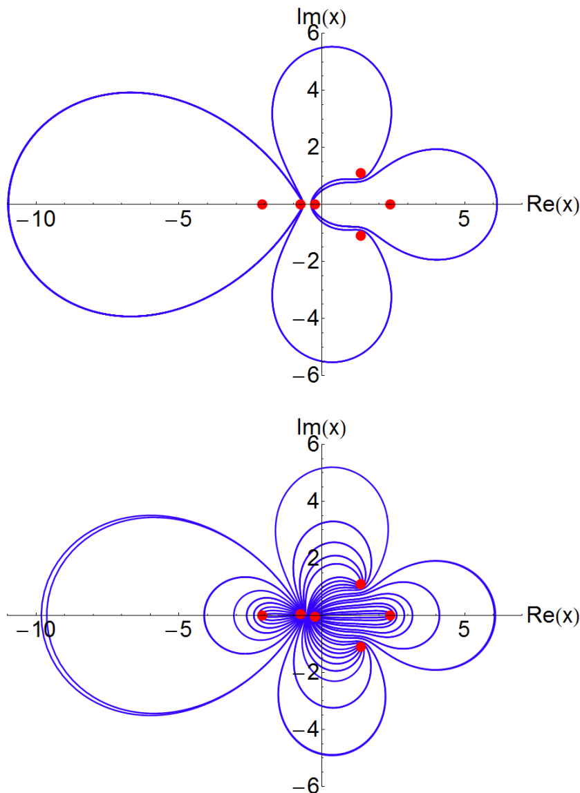
Figure 6. Complex classical trajectories for a particle subject to the sextic potential (2). The energy of the particle in the upper panel is real and three closed nonintersecting trajectories for this particle are shown. The energy of the particle in the lower panel is complex and a single open trajectory is plotted.
