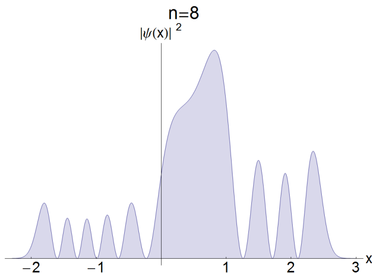
Figure 7. Quantum probability density for a particle in the \psi_8(x) eigenstate in the quartic potential (1) with \hbar = 1/2 . The energy of the particle is E_8 = 3.7239 . The probability density has eight nodes. Note that the particle is most likely to be found inside or near the classically forbidden region associated with the barrier; this shows that the particle does not have a high enough quantum number for its behavior to resemble that of a classical particle.
