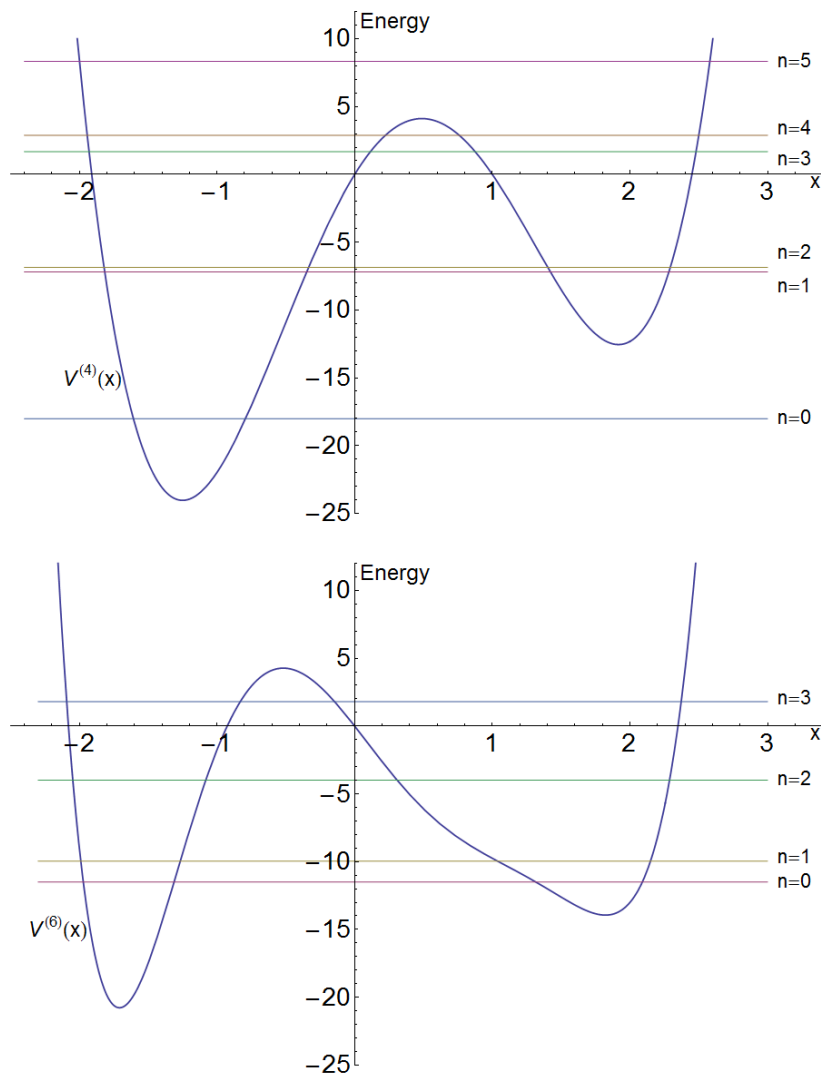
Figure 1. Upper panel: Quartic asymmetric double-well potential V^{(4)}(x) in (1) and the first six quantum energy levels. There are minima at x = -1.2499 , where V^{(4)} = -24.0384 , and at x = 1.9165 , where V^{(4)} = -12.5501 . The peak of the barrier is at x = 0.4884 , where V^{(4)} = 4.1144 . The ground-state energy E_0 lies below the bottom of the right potential well. The next four energy levels lie between the bottom of the right potential well and the top of the barrier. The sixth energy level E_5 lies above the barrier. Lower panel: Sextic asymmetric double-well potential V^{(6)}(x) in (2). The minima of the wells are at x = -1.7083 , where V^{(6)} = -20.7710 , and at x = 1.8215 , where V^{(6)} = -13.9373 . The peak of the barrier is located at x = -0.5184 , where V^{(6)} = 4.2731 .
