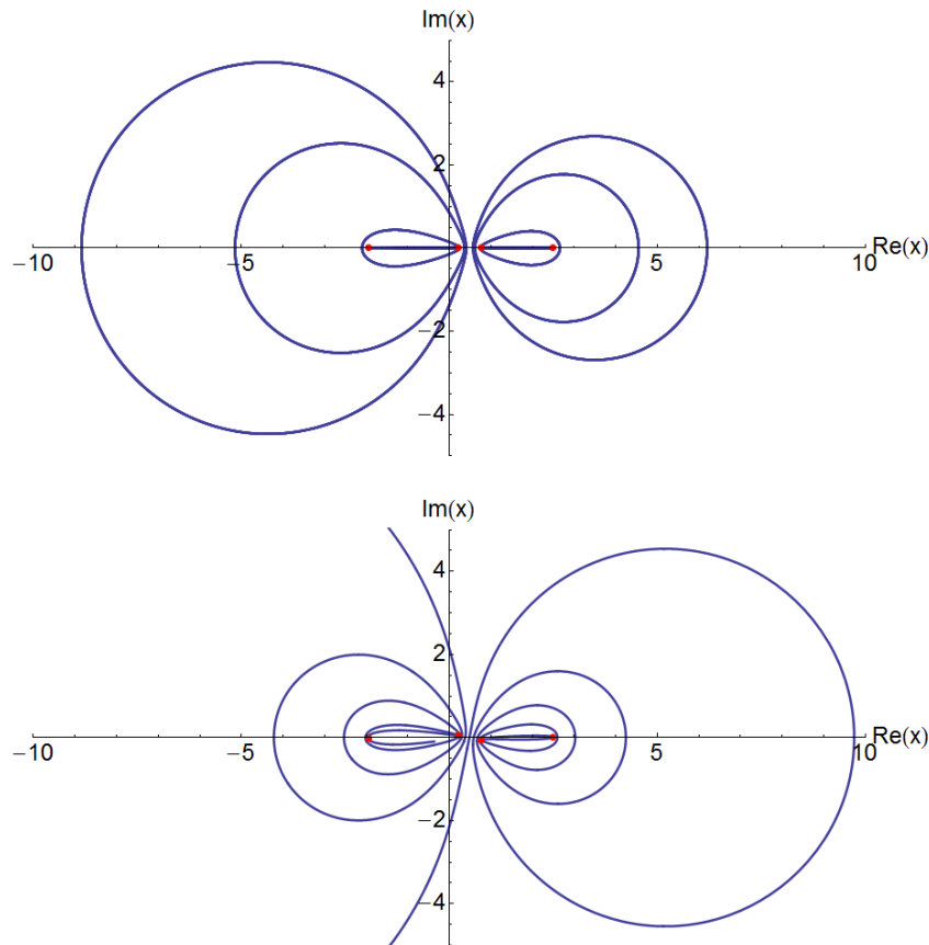
Figure 3. Upper panel: Periodic trajectories in the complex- x plane of a classical particle of real energy E_4 = 2.8845 in the quartic potential (1). The dots indicate the four turning points. There is no tunneling-like behavior; no trajectory runs from one classically allowed region to the other. Lower panel: Classical trajectory in the complex- x plane of a particle of complex energy E = 2.8845 + 0.5i in the same potential (1). Unlike the closed trajectories in the upper panel, this classical trajectory is open. The particle begins at x = 1 and traces an outward anticlockwise spiral around the right pair of turning points. It then crosses to the left of the peak of the barrier and spirals inward and clockwise around the left pair of turning points. Next, it crosses the real axis between the left turning points and spirals outward and anticlockwise around the left pair of turning points. The time for the displayed trajectory is t = 8 . For t > 8 , the particle continues to spiral inward and outward as it oscillates from well to well. The particle exhibits this deterministic tunneling-like behavior for all time, but the trajectory never crosses itself. This trajectory behaves as if it were controlled by a pair of strange attractors.
