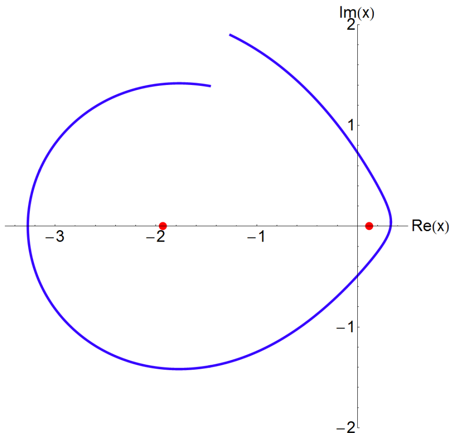
Figure 4. Complex path of a particle of complex energy E = 2.8845 + 0.25i . The time of this path is taken to be t = T = 0.8464 , which is the same as the period of a classical particle of real energy E = 2.8845 . Note that the particle in this figure makes an approximately full angular revolution around the two turning points, which are denoted by dots. However, the path is not closed.
