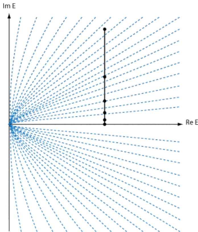
Figure 5. Schematic drawing of the special complex energies for which the particle motion in the quartic potential (1) is periodic for any choice of initial condition. These energies lie on asymptotically straight dashed curves that approach the origin in the complex- E plane. The energies form a set of measure zero; there are an infinite number of such curves and these curves are dense in the complex- E plane. The regulation procedure used in this paper establishes a connection between complex classical mechanics and quantum mechanics by taking a sequence of complex classical energies in which the imaginary part tends to 0. This sequence is indicated by dots on the solid vertical line. Although this line intersects the dashed lines infinitely many times, the numerical procedure remains unaffected.
